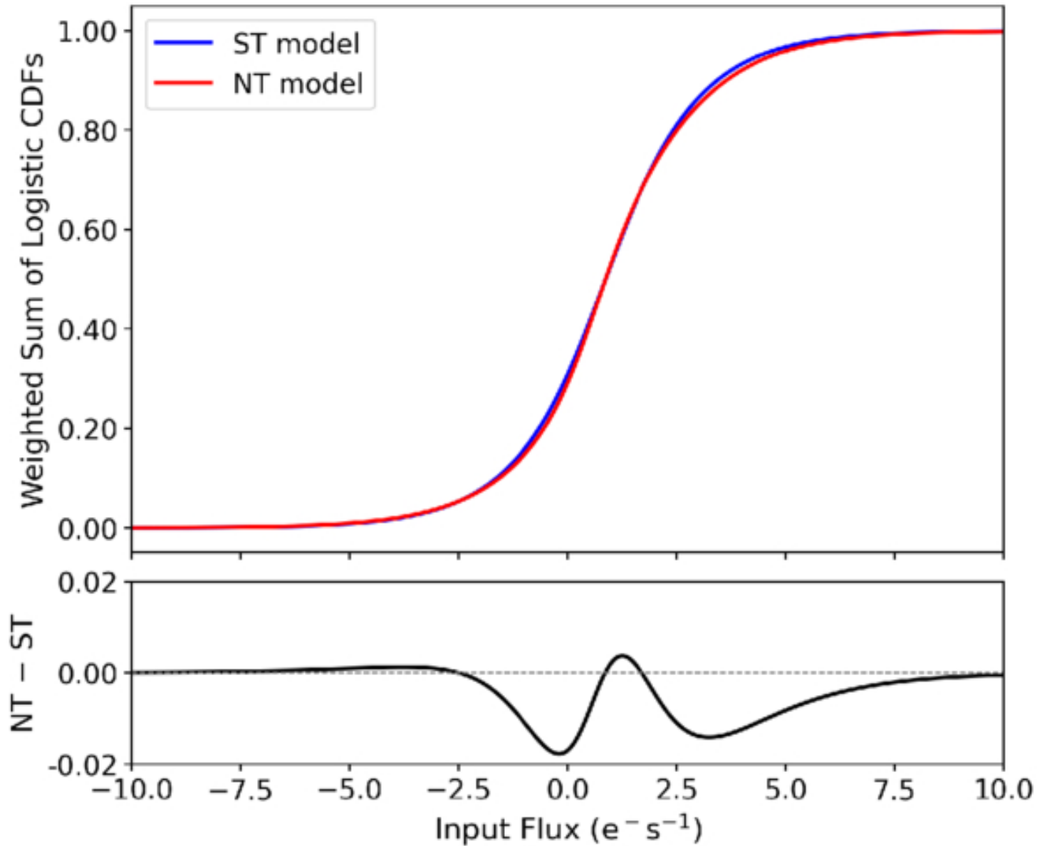
Figure 7. from Brian P. Powell et al 2026 Astron. J. 172 doi:10.3847/1538-3881/ae6cfc https://dx.doi.org/10.3847/1538-3881/ae6cfc © 2026. The Author(s). Published by the American Astronomical Society.
