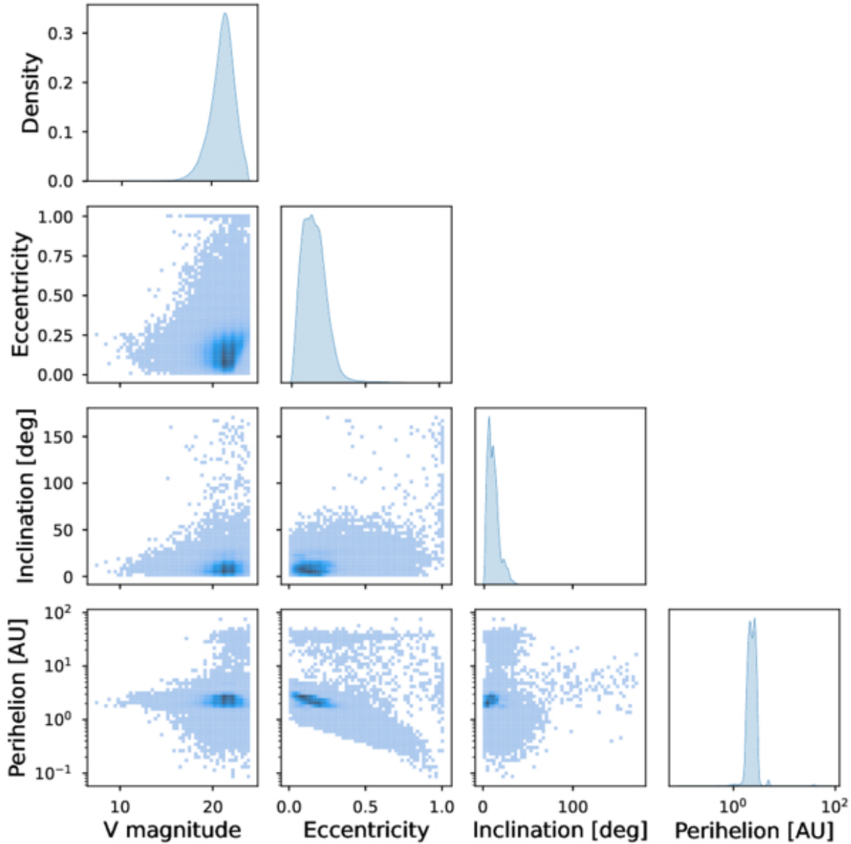
Figure 2. from Brian P. Powell et al 2026 Astron. J. 172 doi:10.3847/1538-3881/ae6cfc https://dx.doi.org/10.3847/1538-3881/ae6cfc © 2026. The Author(s). Published by the American Astronomical Society.
