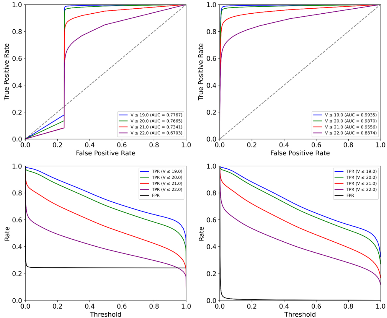
Figure 14. from Brian P. Powell et al 2026 Astron. J. 172 doi:10.3847/1538-3881/ae6cfc https://dx.doi.org/10.3847/1538-3881/ae6cfc © 2026. The Author(s). Published by the American Astronomical Society.
