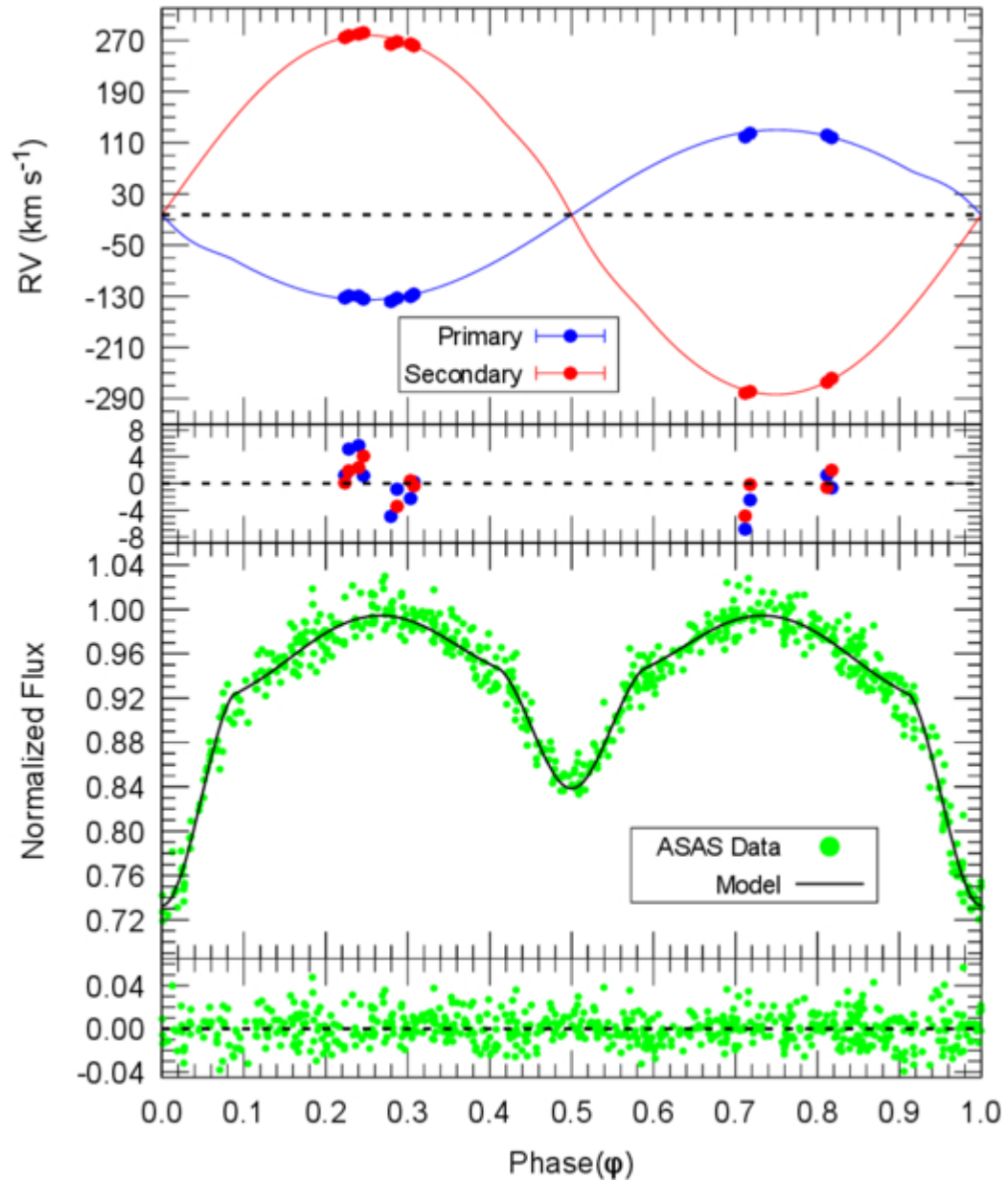
Figure 3. from Gökhan Yücel et al 2026 Astron. J. 172 doi:10.3847/1538-3881/ae6cfb https://dx.doi.org/10.3847/1538-3881/ae6cfb © 2026. The Author(s). Published by the American Astronomical Society.
