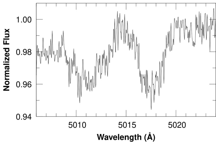
5015.678 Å He I
