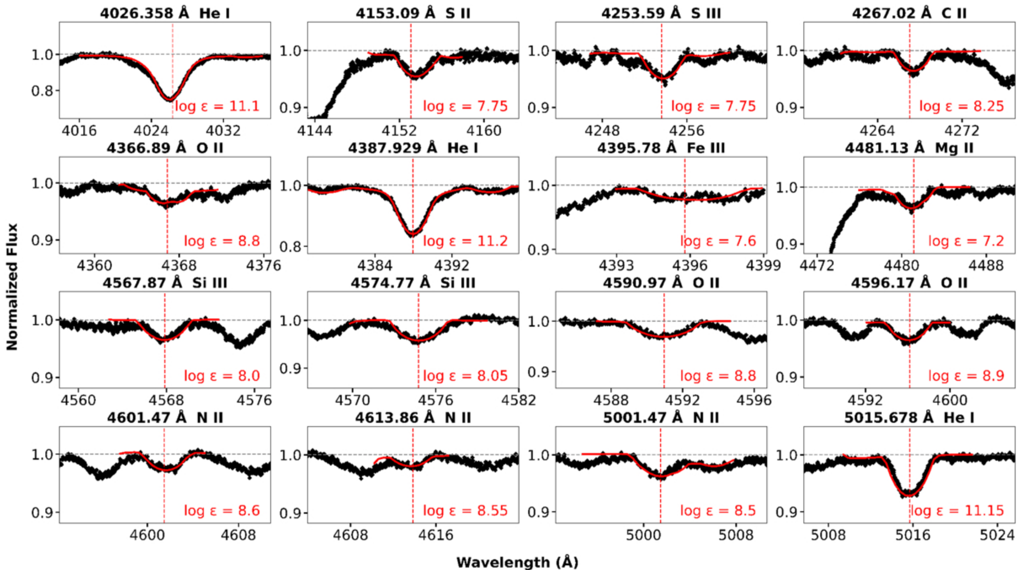
Figure 10. from Gökhan Yücel et al 2026 Astron. J. 172 doi:10.3847/1538-3881/ae6cfb https://dx.doi.org/10.3847/1538-3881/ae6cfb © 2026. The Author(s). Published by the American Astronomical Society.
