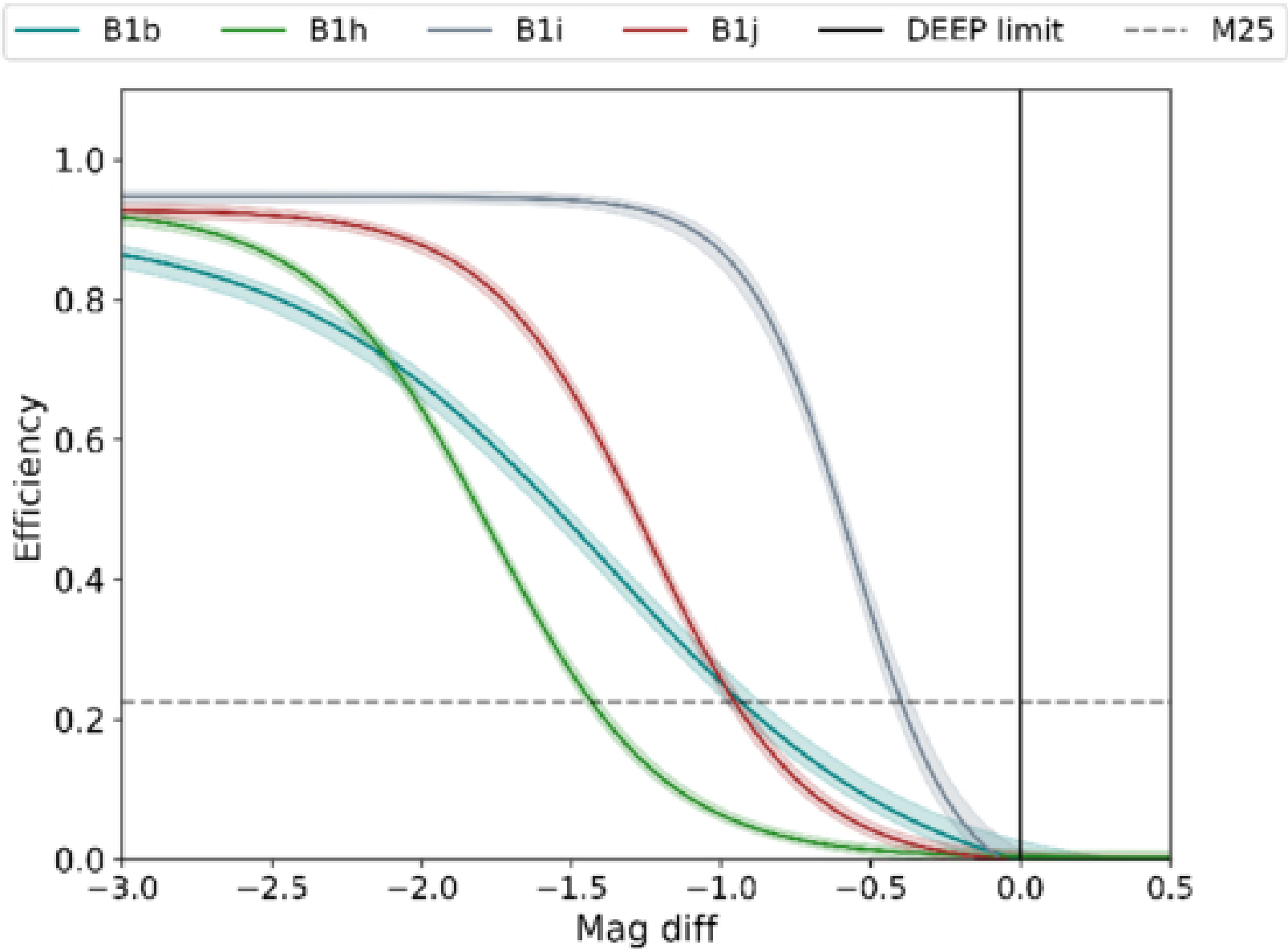
Figure 7. from Nitya Pandey et al 2026 Astron. J. 172 doi:10.3847/1538-3881/ae6cf4 https://dx.doi.org/10.3847/1538-3881/ae6cf4 © 2026. The Author(s). Published by the American Astronomical Society.
