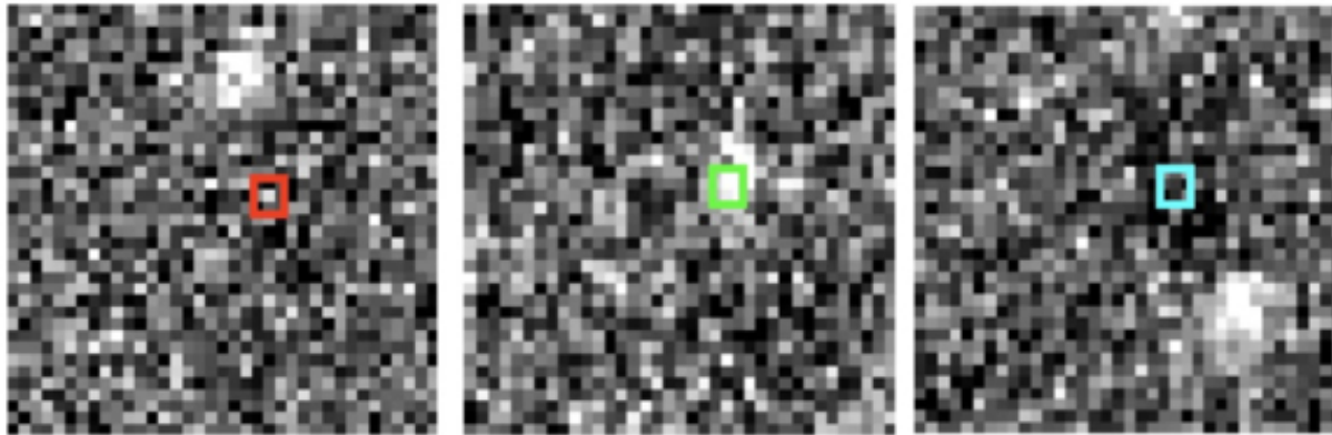
Figure 2. from Nitya Pandey et al 2026 Astron. J. 172 doi:10.3847/1538-3881/ae6cf4 https://dx.doi.org/10.3847/1538-3881/ae6cf4 © 2026. The Author(s). Published by the American Astronomical Society.
