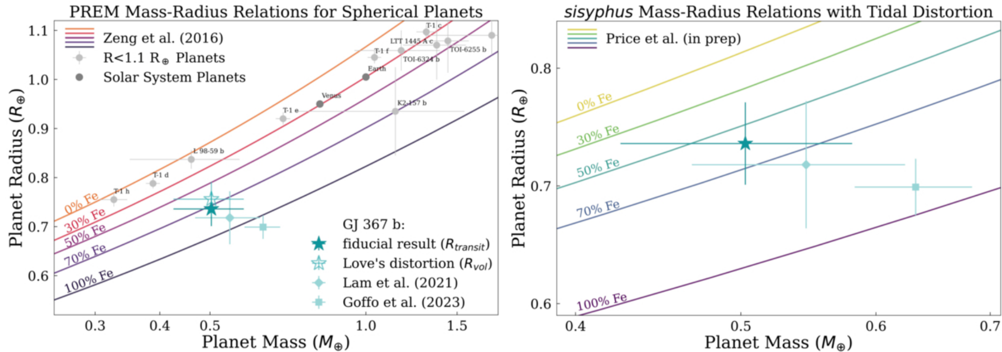
Figure 3. from Rena A. Lee et al 2026 Astron. J. 172 doi:10.3847/1538-3881/ae6cec https://dx.doi.org/10.3847/1538-3881/ae6cec © 2026. The Author(s). Published by the American Astronomical Society.
