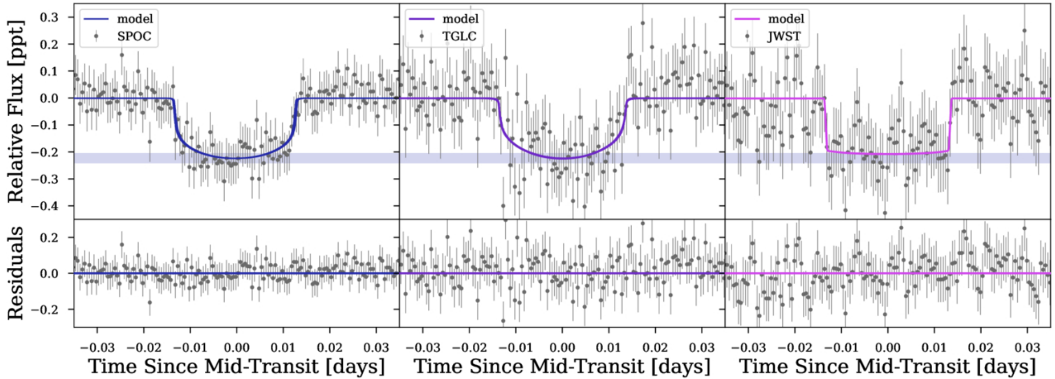
Figure 1. from Rena A. Lee et al 2026 Astron. J. 172 doi:10.3847/1538-3881/ae6cec https://dx.doi.org/10.3847/1538-3881/ae6cec © 2026. The Author(s). Published by the American Astronomical Society.
