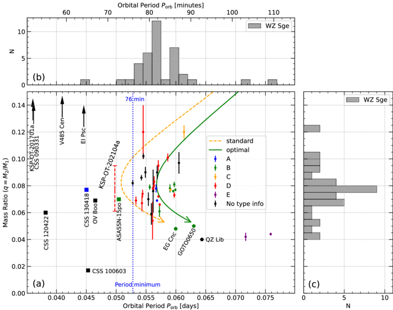
Figure 8. from Sang Chul Kim et al 2026 Astron. J. 172 doi:10.3847/1538-3881/ae6b7f https://dx.doi.org/10.3847/1538-3881/ae6b7f © 2026. The Author(s). Published by the American Astronomical Society.
