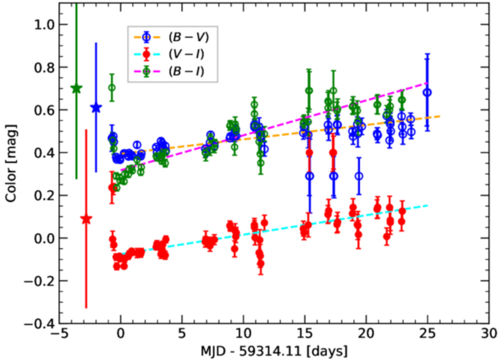
Figure 6. from Sang Chul Kim et al 2026 Astron. J. 172 doi:10.3847/1538-3881/ae6b7f https://dx.doi.org/10.3847/1538-3881/ae6b7f © 2026. The Author(s). Published by the American Astronomical Society.
