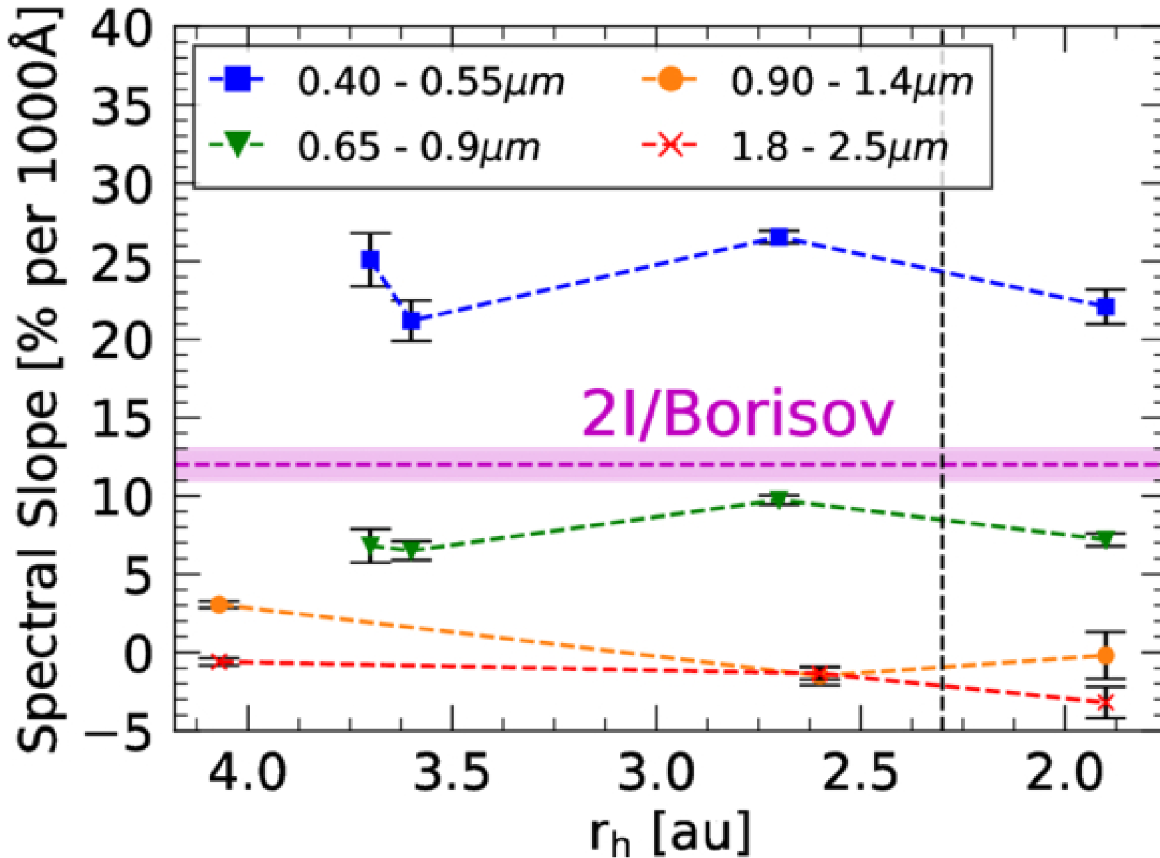
Figure 3. from Kyle Medler et al 2026 Astron. J. 172 doi:10.3847/1538-3881/ae6b71 https://dx.doi.org/10.3847/1538-3881/ae6b71 © 2026. The Author(s). Published by the American Astronomical Society.
