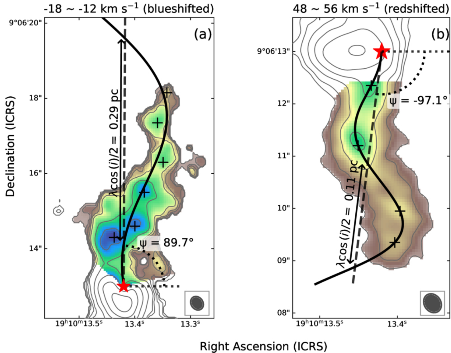
Figure 4. from Yunfan Jiao et al 2026 Astron. J. 172 doi:10.3847/1538-3881/ae6b6d https://dx.doi.org/10.3847/1538-3881/ae6b6d © 2026. The Author(s). Published by the American Astronomical Society.
