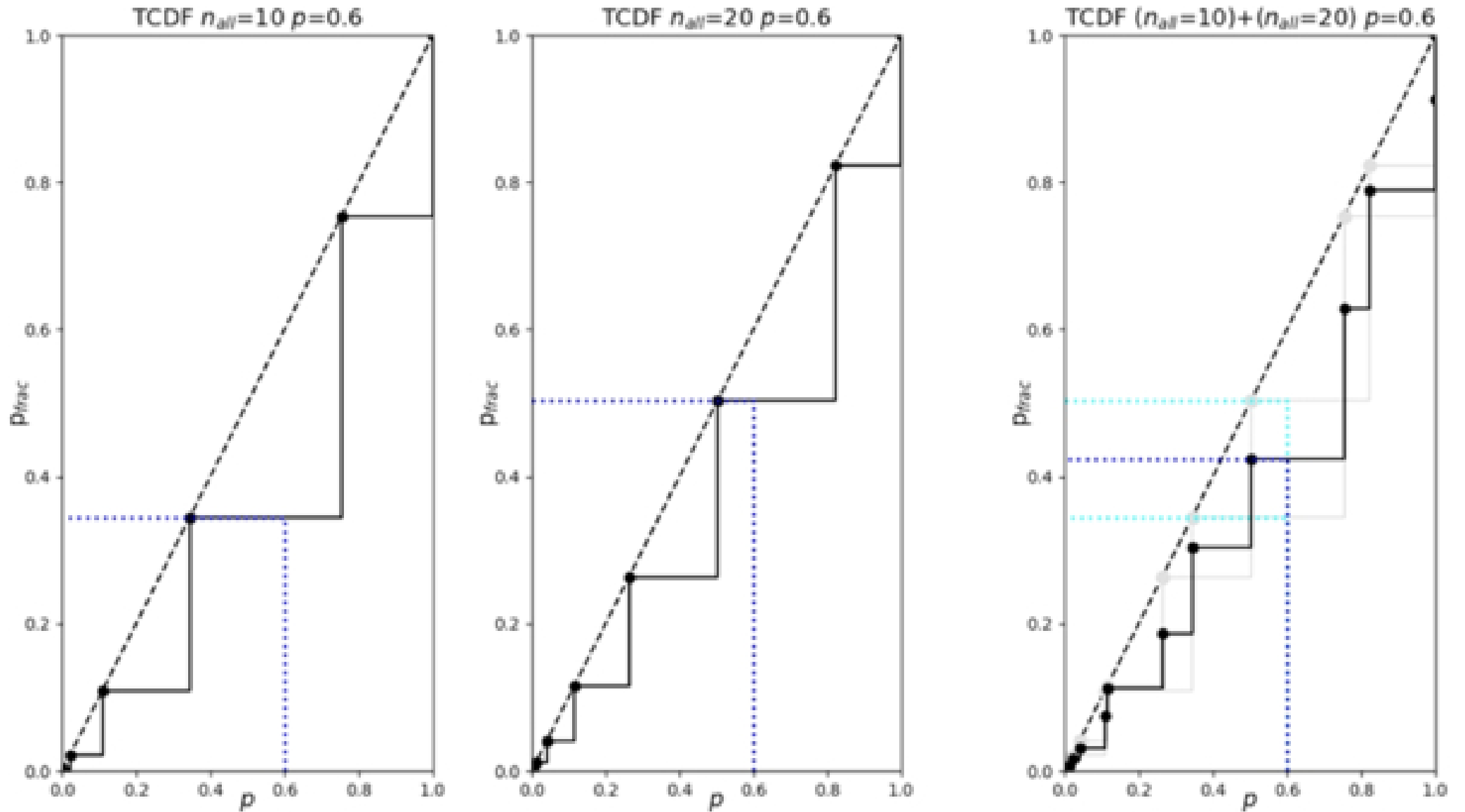
Figure 3. from Masanori Iye and Masafumi Yagi 2026 Astron. J. 172 doi:10.3847/1538-3881/ae6a99 https://dx.doi.org/10.3847/1538-3881/ae6a99 © 2026. The Author(s). Published by the American Astronomical Society.
