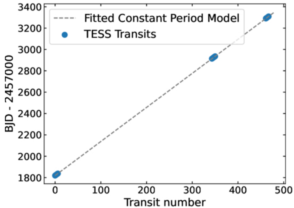
Figure 2. from Raven Cilley et al 2026 Astron. J. 171 doi:10.3847/1538-3881/ae69d4 https://dx.doi.org/10.3847/1538-3881/ae69d4 © 2026. The Author(s). Published by the American Astronomical Society.
