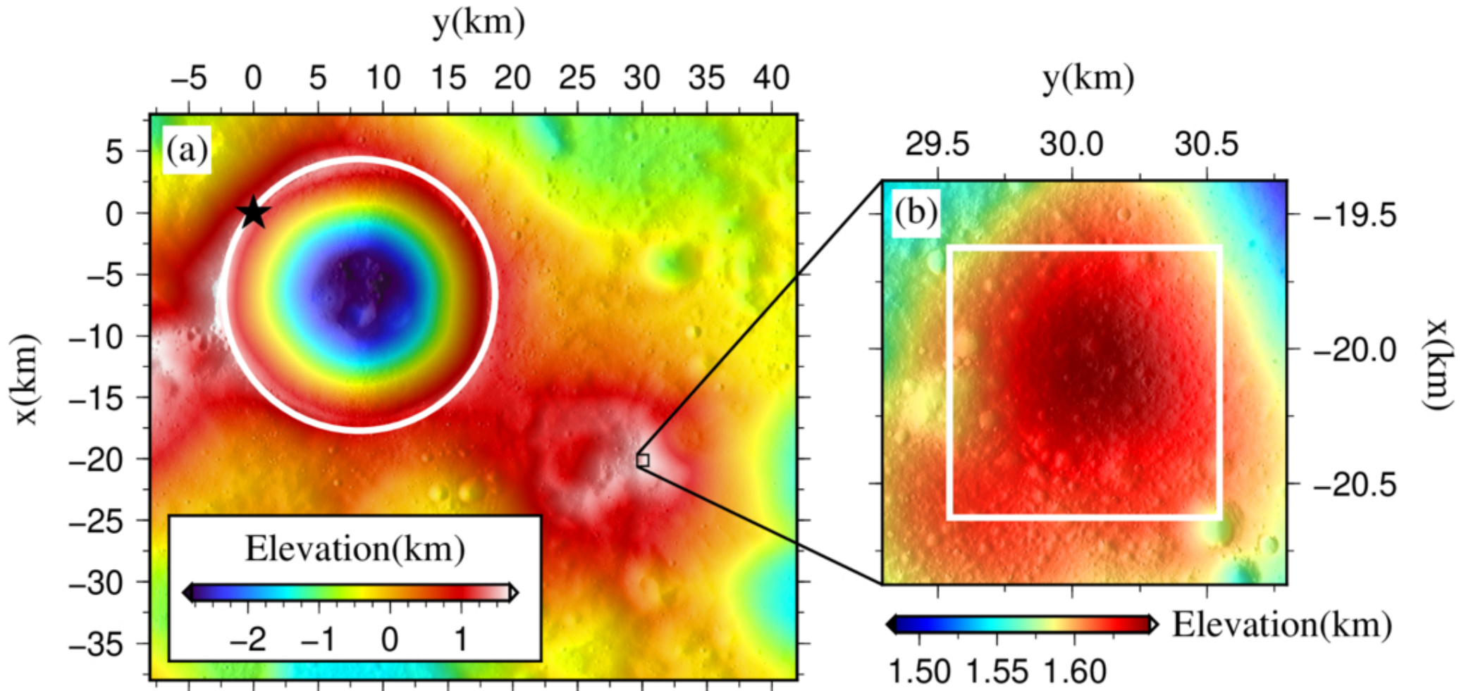
Figure 1. from Zhen Zhong et al 2026 Astron. J. 171 doi:10.3847/1538-3881/ae6918 https://dx.doi.org/10.3847/1538-3881/ae6918 © 2026. The Author(s). Published by the American Astronomical Society.
