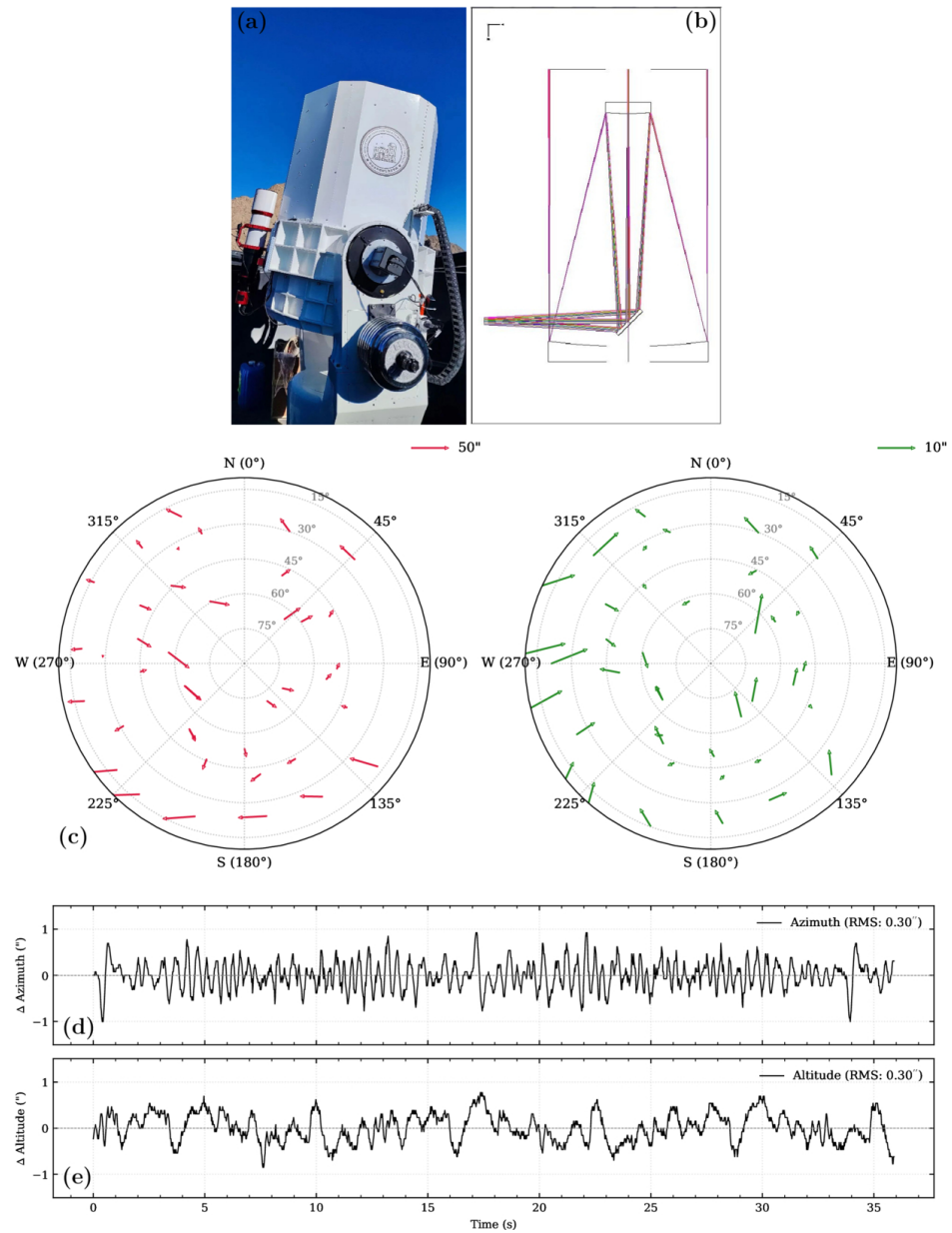
Figure 1. from Zhong-Nan Dong et al 2026 Astron. J. 171 doi:10.3847/1538-3881/ae6802 https://dx.doi.org/10.3847/1538-3881/ae6802 © 2026. The Author(s). Published by the American Astronomical Society.
