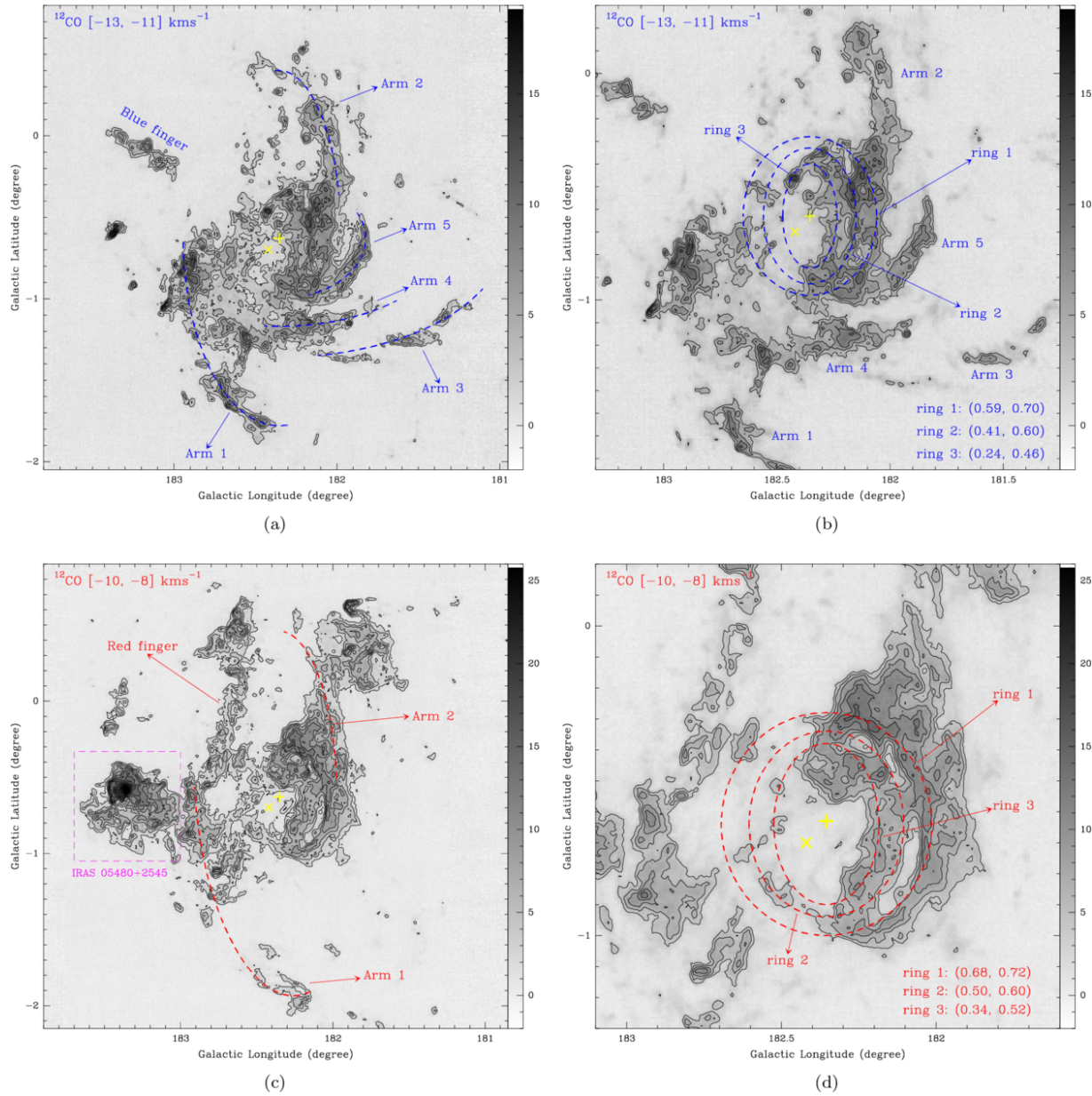
Figure 2. from Xuepeng Chen et al 2026 Astron. J. 172 doi:10.3847/1538-3881/ae6800 https://dx.doi.org/10.3847/1538-3881/ae6800 © 2026. The Author(s). Published by the American Astronomical Society.
