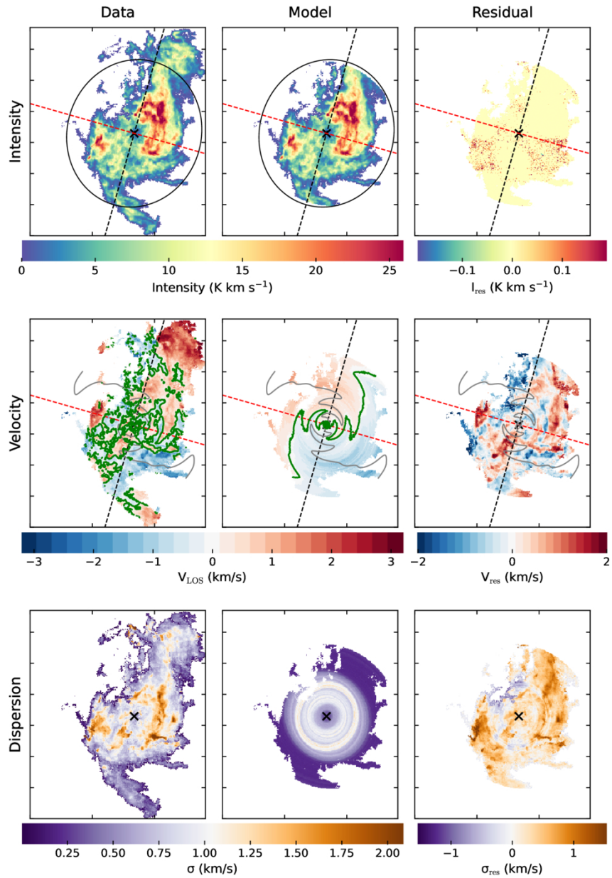
Figure 14. from Xuepeng Chen et al 2026 Astron. J. 172 doi:10.3847/1538-3881/ae6800 https://dx.doi.org/10.3847/1538-3881/ae6800 © 2026. The Author(s). Published by the American Astronomical Society.
