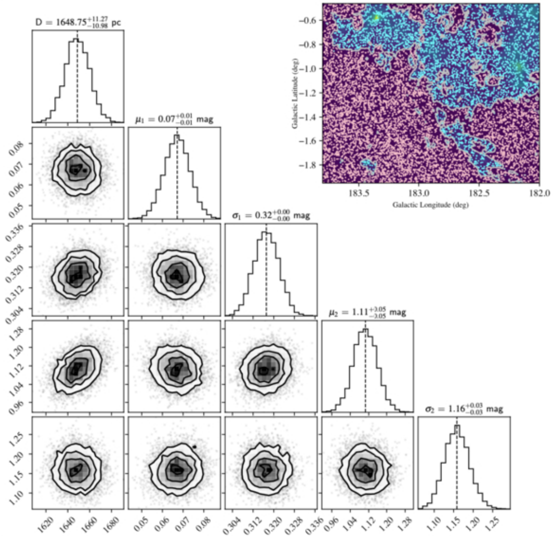
Figure 12. from Xuepeng Chen et al 2026 Astron. J. 172 doi:10.3847/1538-3881/ae6800 https://dx.doi.org/10.3847/1538-3881/ae6800 © 2026. The Author(s). Published by the American Astronomical Society.
