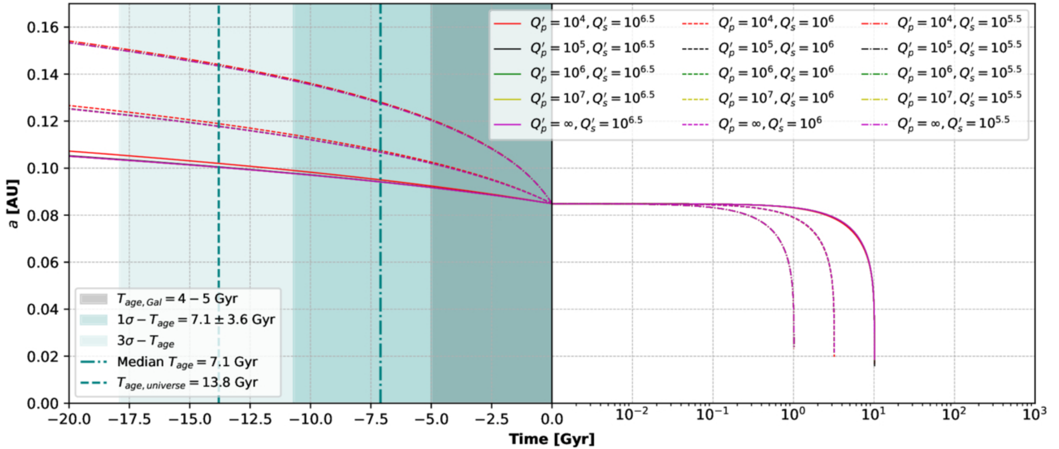
Figure 8. from Rohan Ch. Das et al 2026 Astron. J. 171 doi:10.3847/1538-3881/ae66ff https://dx.doi.org/10.3847/1538-3881/ae66ff © 2026. The Author(s). Published by the American Astronomical Society.
