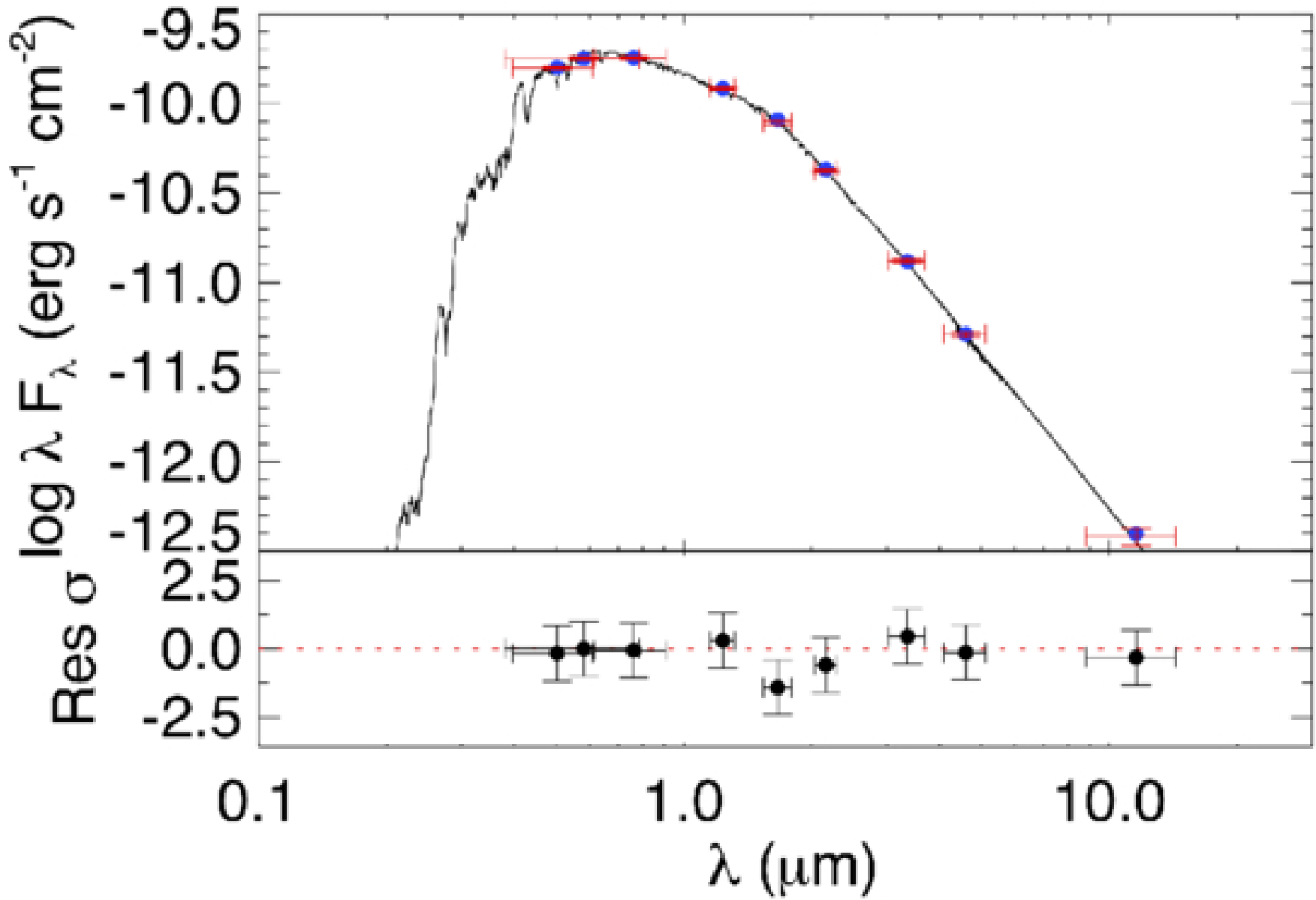
Figure 5. from Rohan Ch. Das et al 2026 Astron. J. 171 doi:10.3847/1538-3881/ae66ff https://dx.doi.org/10.3847/1538-3881/ae66ff © 2026. The Author(s). Published by the American Astronomical Society.
