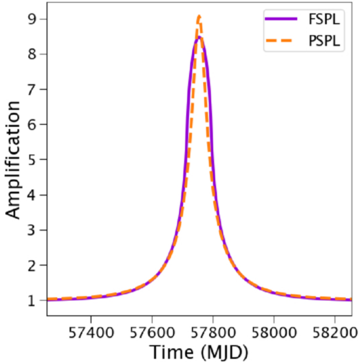
Figure 6. from J. R. Lu et al 2026 Astron. J. 172 doi:10.3847/1538-3881/ae665b https://dx.doi.org/10.3847/1538-3881/ae665b © 2026. The Author(s). Published by the American Astronomical Society.
