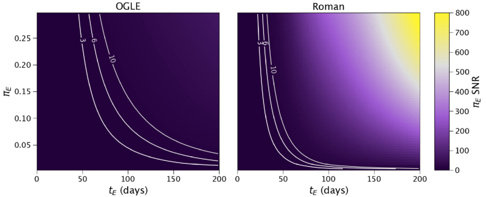
Figure 17. from J. R. Lu et al 2026 Astron. J. 172 doi:10.3847/1538-3881/ae665b https://dx.doi.org/10.3847/1538-3881/ae665b © 2026. The Author(s). Published by the American Astronomical Society.
