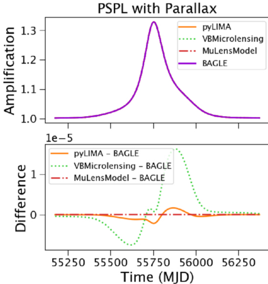
Figure 10. from J. R. Lu et al 2026 Astron. J. 172 doi:10.3847/1538-3881/ae665b https://dx.doi.org/10.3847/1538-3881/ae665b © 2026. The Author(s). Published by the American Astronomical Society.
