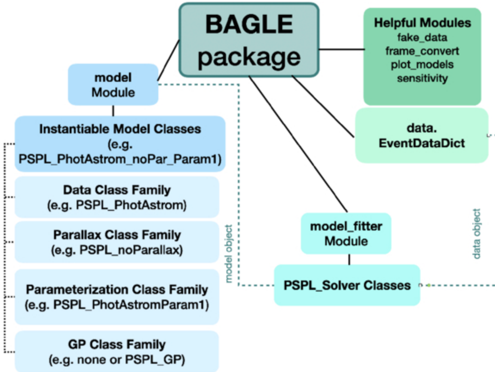
Figure 1. from J. R. Lu et al 2026 Astron. J. 172 doi:10.3847/1538-3881/ae665b https://dx.doi.org/10.3847/1538-3881/ae665b © 2026. The Author(s). Published by the American Astronomical Society.
