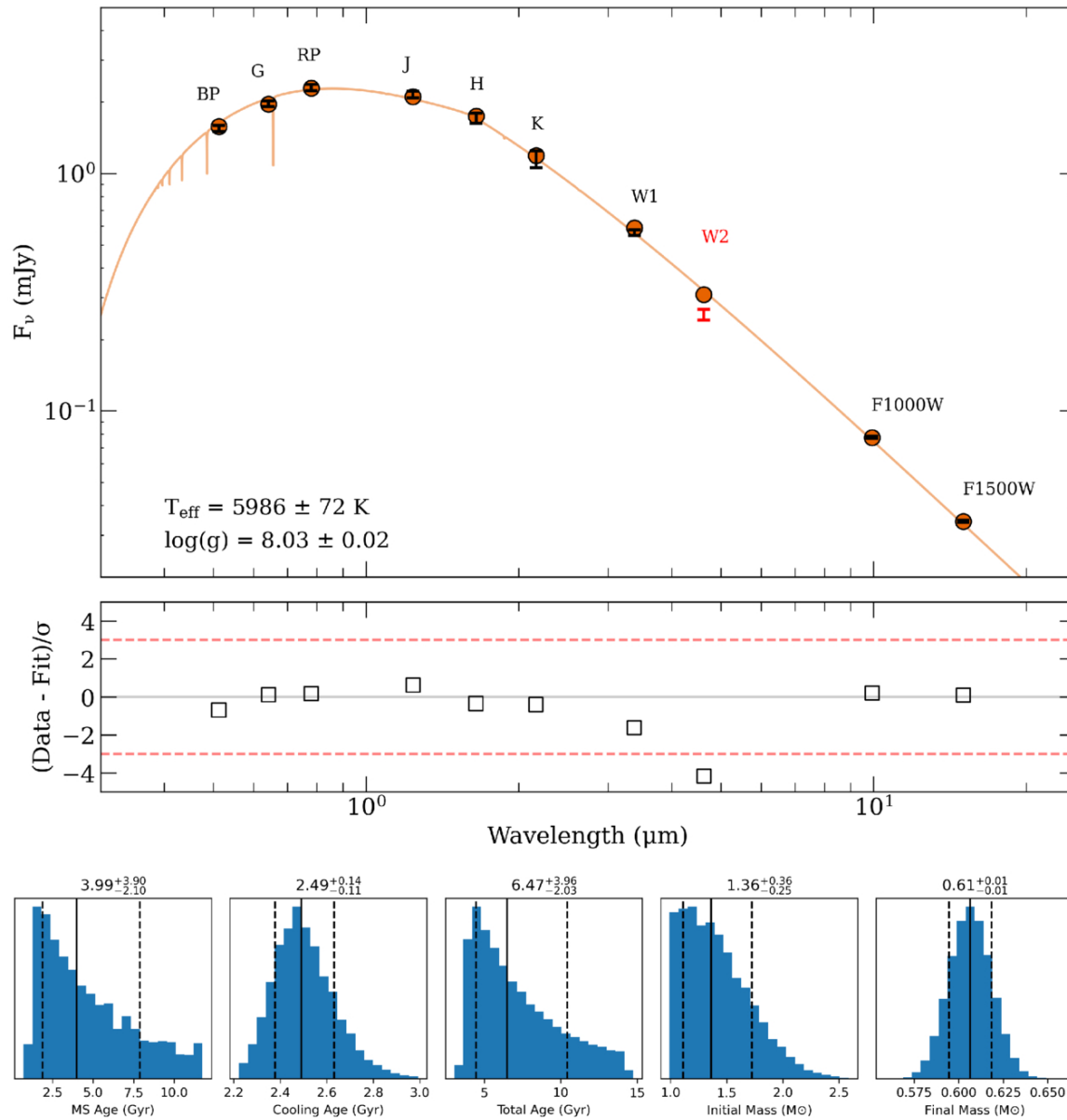
Figure 4. from Loïc Albert et al 2026 Astron. J. 171 doi:10.3847/1538-3881/ae650d https://dx.doi.org/10.3847/1538-3881/ae650d © 2026. The Author(s). Published by the American Astronomical Society.
