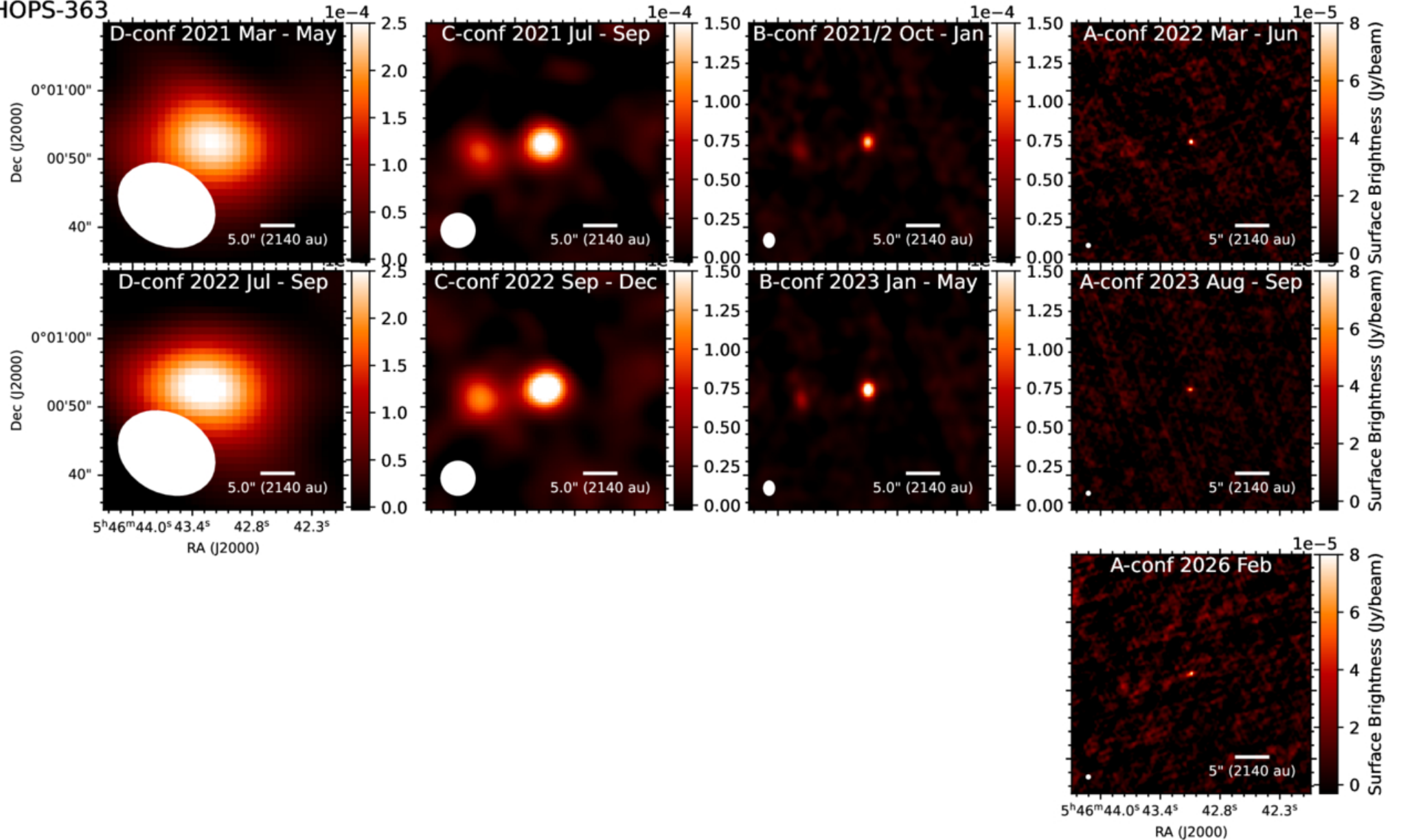
Figure 8. from John J. Tobin et al 2026 Astron. J. 172 doi:10.3847/1538-3881/ae6502 https://dx.doi.org/10.3847/1538-3881/ae6502 © 2026. The Author(s). Published by the American Astronomical Society.
