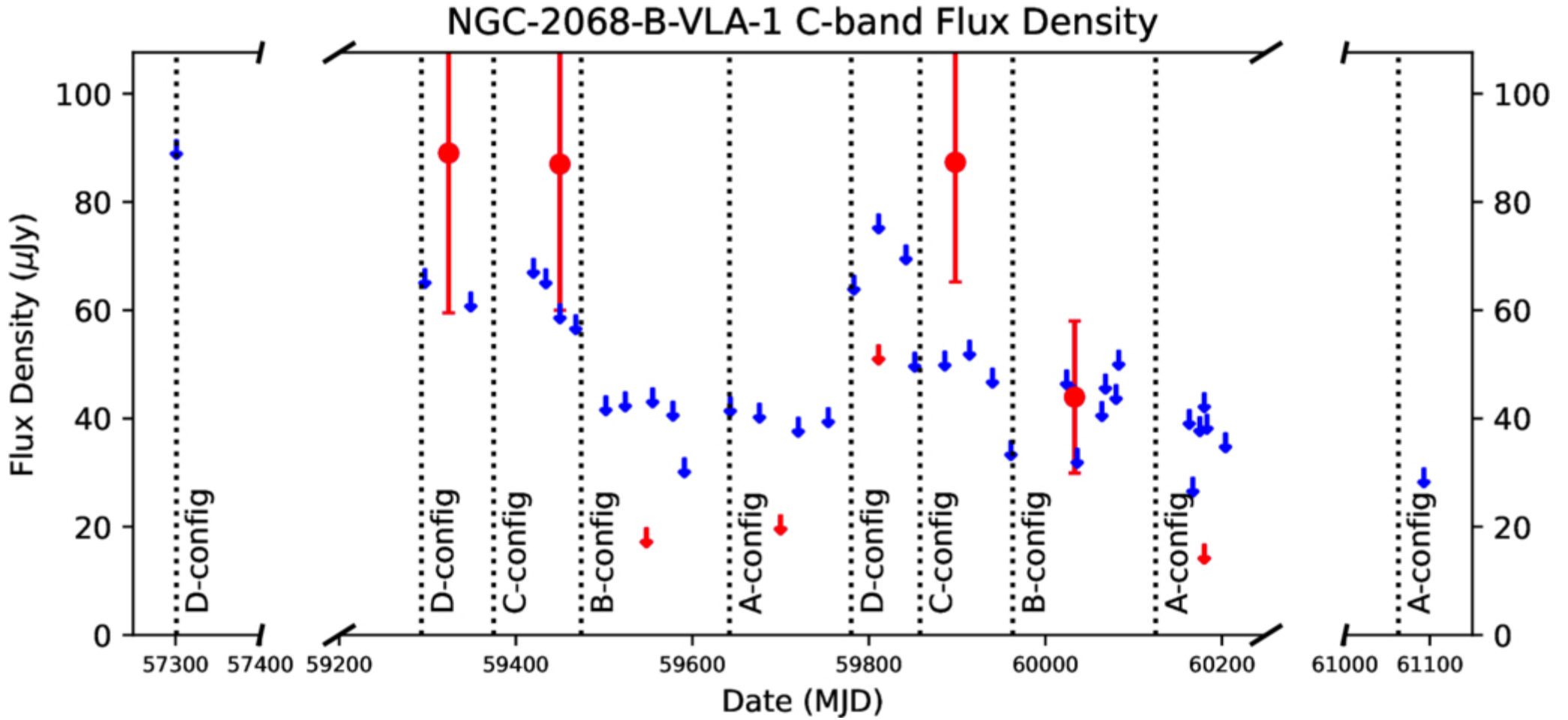
Figure 16. Time Series Plots for All Sources from John J. Tobin et al 2026 Astron. J. 172 doi:10.3847/1538-3881/ae6502 https://dx.doi.org/10.3847/1538-3881/ae6502 © 2026. The Author(s). Published by the American Astronomical Society.
