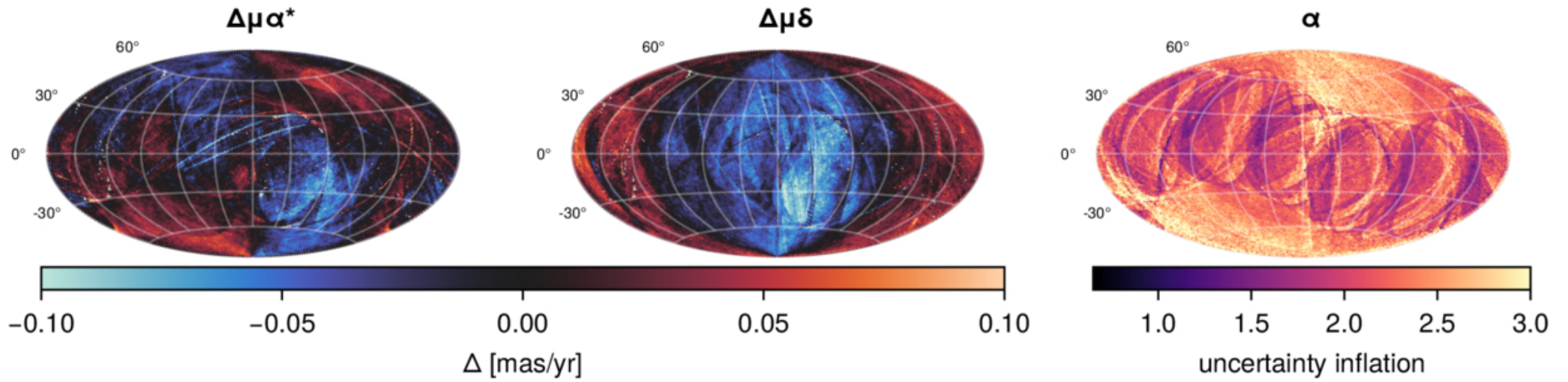
Figure 2. from William Thompson et al 2026 Astron. J. 172 doi:10.3847/1538-3881/ae64ed https://dx.doi.org/10.3847/1538-3881/ae64ed © 2026. The Author(s). Published by the American Astronomical Society.
