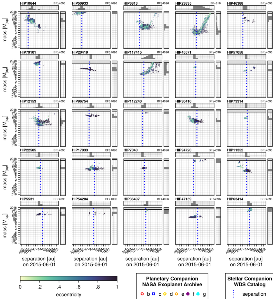
Figure 14. from William Thompson et al 2026 Astron. J. 172 doi:10.3847/1538-3881/ae64ed https://dx.doi.org/10.3847/1538-3881/ae64ed © 2026. The Author(s). Published by the American Astronomical Society.
