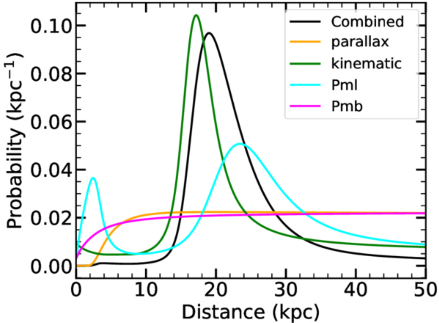
Figure 4. from Xianjin Shen et al 2026 Astron. J. 171 doi:10.3847/1538-3881/ae64e8 https://dx.doi.org/10.3847/1538-3881/ae64e8 © 2026. The Author(s). Published by the American Astronomical Society.
