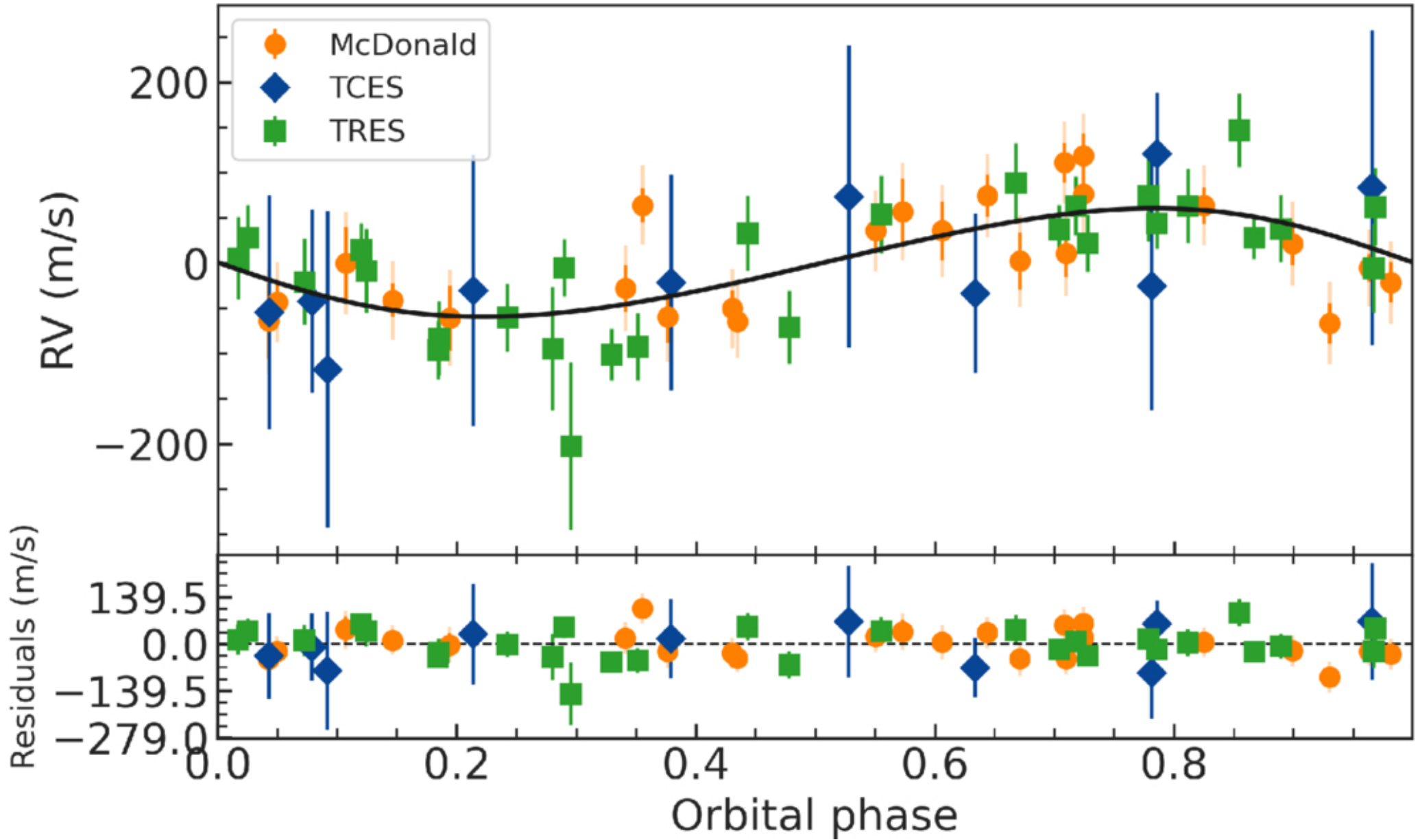
Figure 7. from Eike W. Guenther et al 2026 Astron. J. 172 doi:10.3847/1538-3881/ae6449 https://dx.doi.org/10.3847/1538-3881/ae6449 © 2026. The Author(s). Published by the American Astronomical Society.
