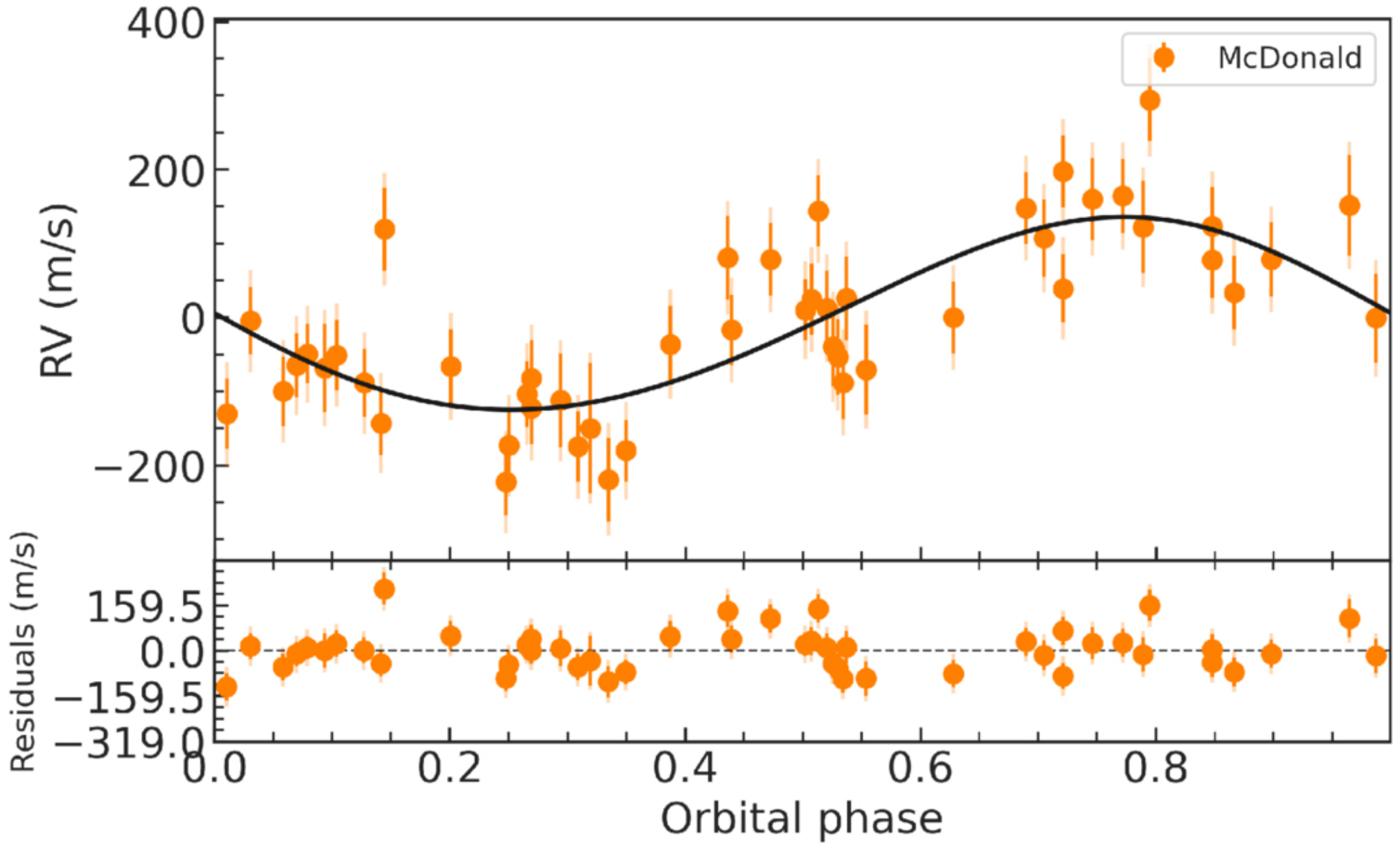
Figure 4. from Eike W. Guenther et al 2026 Astron. J. 172 doi:10.3847/1538-3881/ae6449 https://dx.doi.org/10.3847/1538-3881/ae6449 © 2026. The Author(s). Published by the American Astronomical Society.
