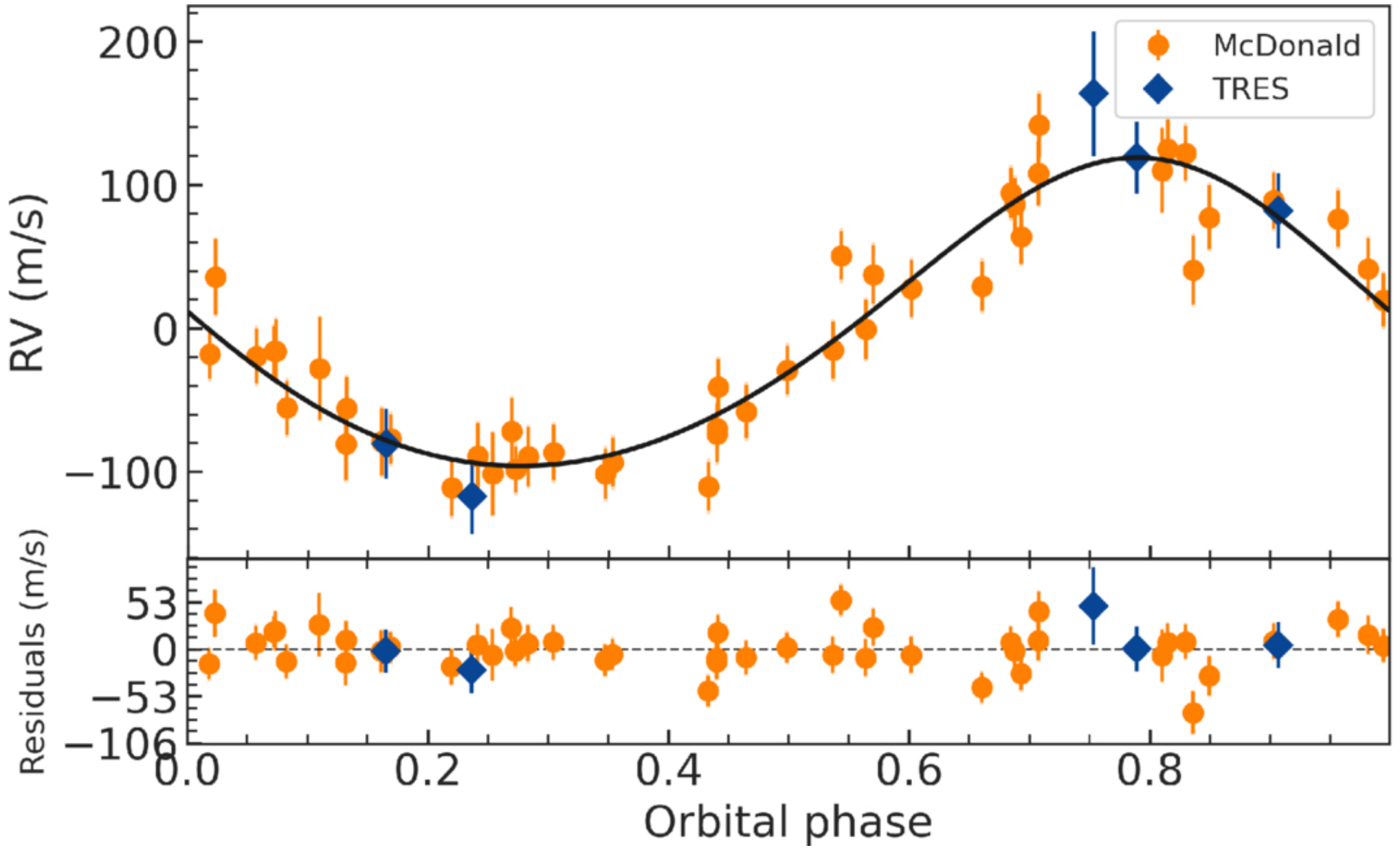
Figure 2. from Eike W. Guenther et al 2026 Astron. J. 172 doi:10.3847/1538-3881/ae6449 https://dx.doi.org/10.3847/1538-3881/ae6449 © 2026. The Author(s). Published by the American Astronomical Society.
