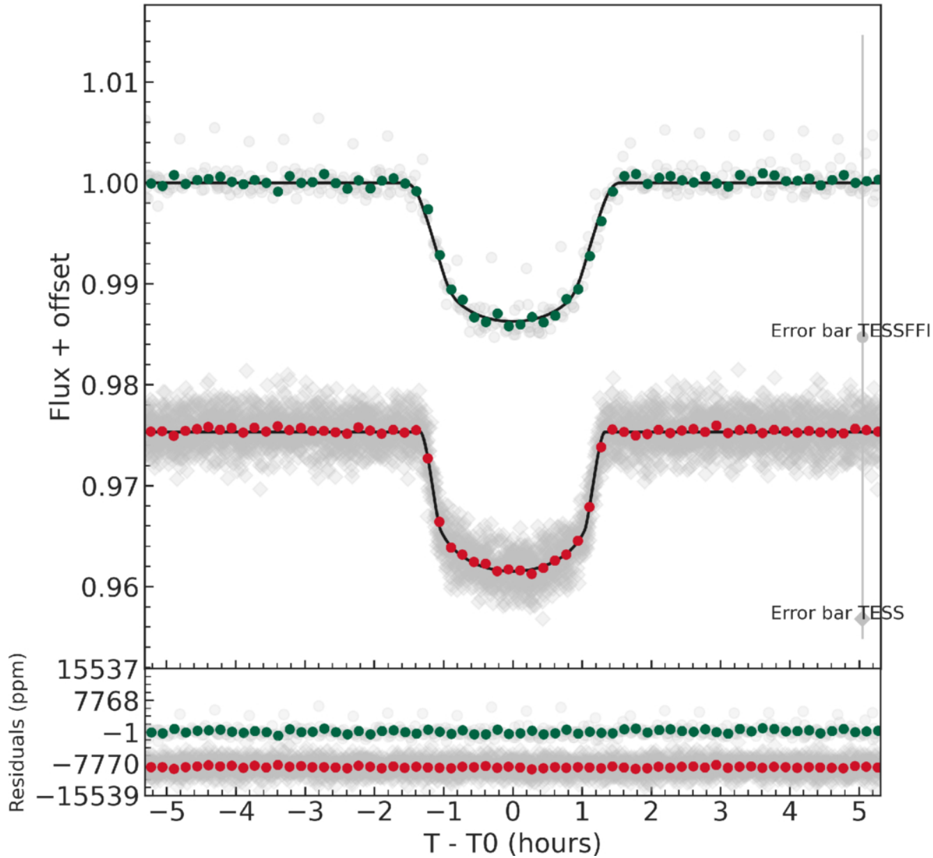
Figure 1. from Eike W. Guenther et al 2026 Astron. J. 172 doi:10.3847/1538-3881/ae6449 https://dx.doi.org/10.3847/1538-3881/ae6449 © 2026. The Author(s). Published by the American Astronomical Society.
