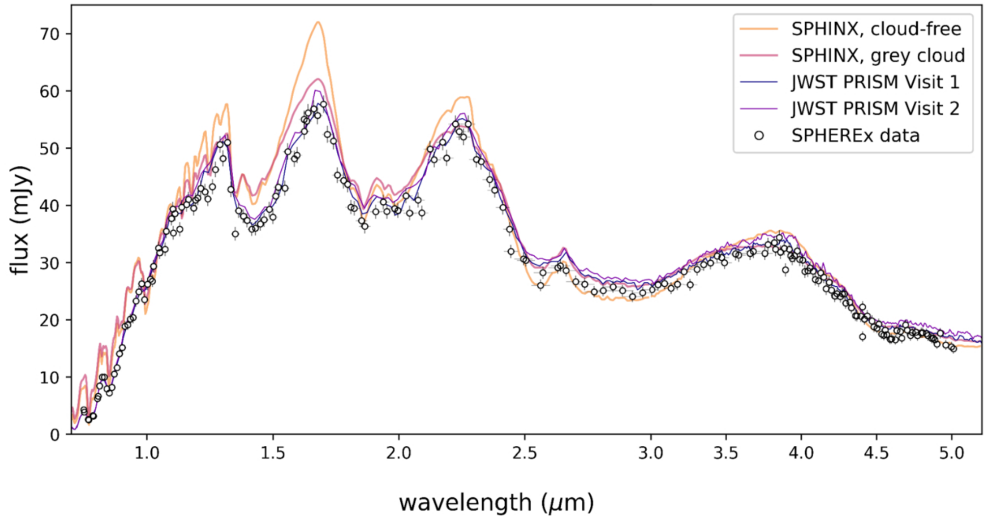
Figure 6. from Catherine A. Clark et al 2026 Astron. J. 172 doi:10.3847/1538-3881/ae63c2 https://dx.doi.org/10.3847/1538-3881/ae63c2 © 2026. The Author(s). Published by the American Astronomical Society.
