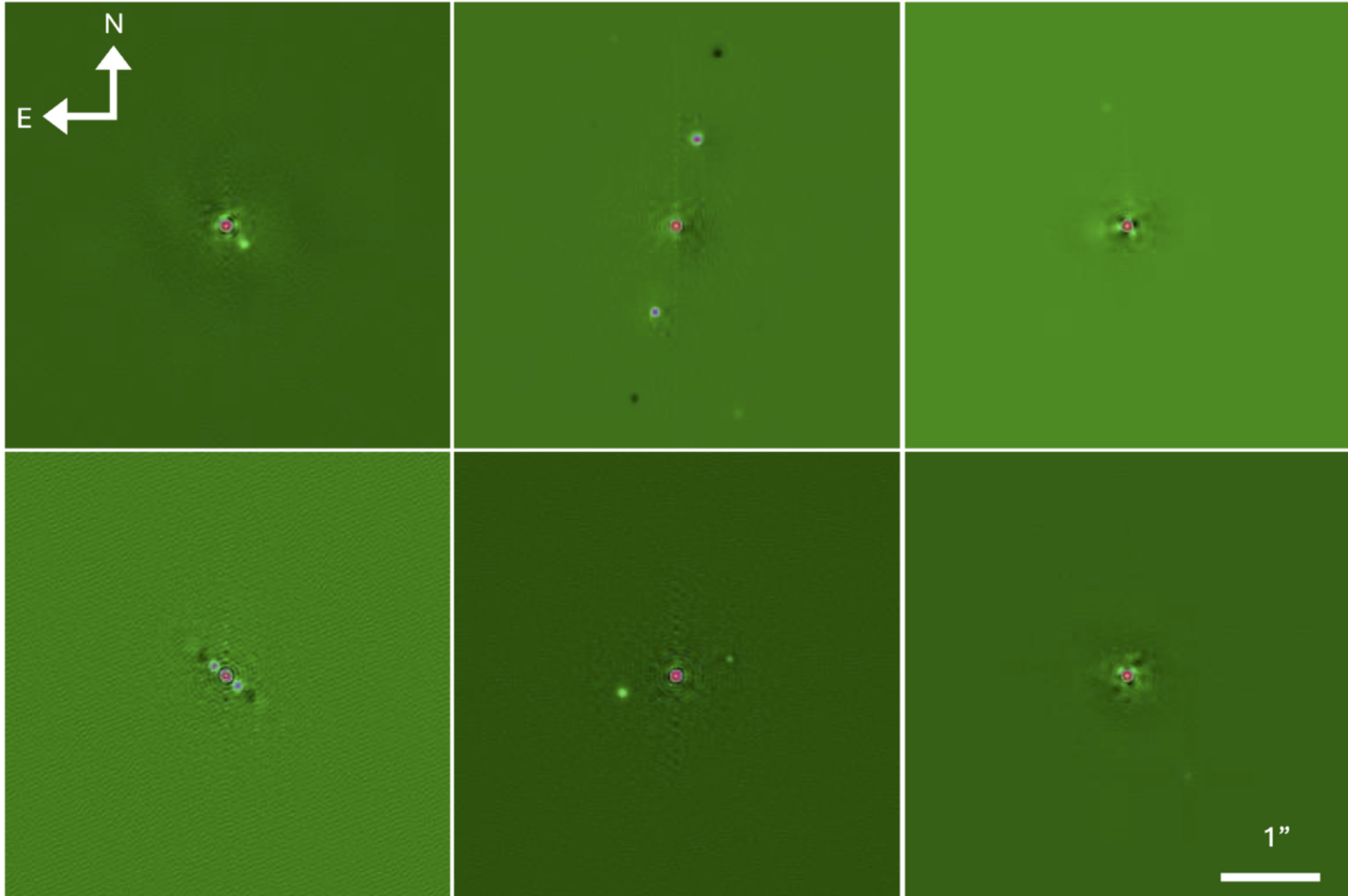
Figure 3. from Catherine A. Clark et al 2026 Astron. J. 172 doi:10.3847/1538-3881/ae63c2 https://dx.doi.org/10.3847/1538-3881/ae63c2 © 2026. The Author(s). Published by the American Astronomical Society.
