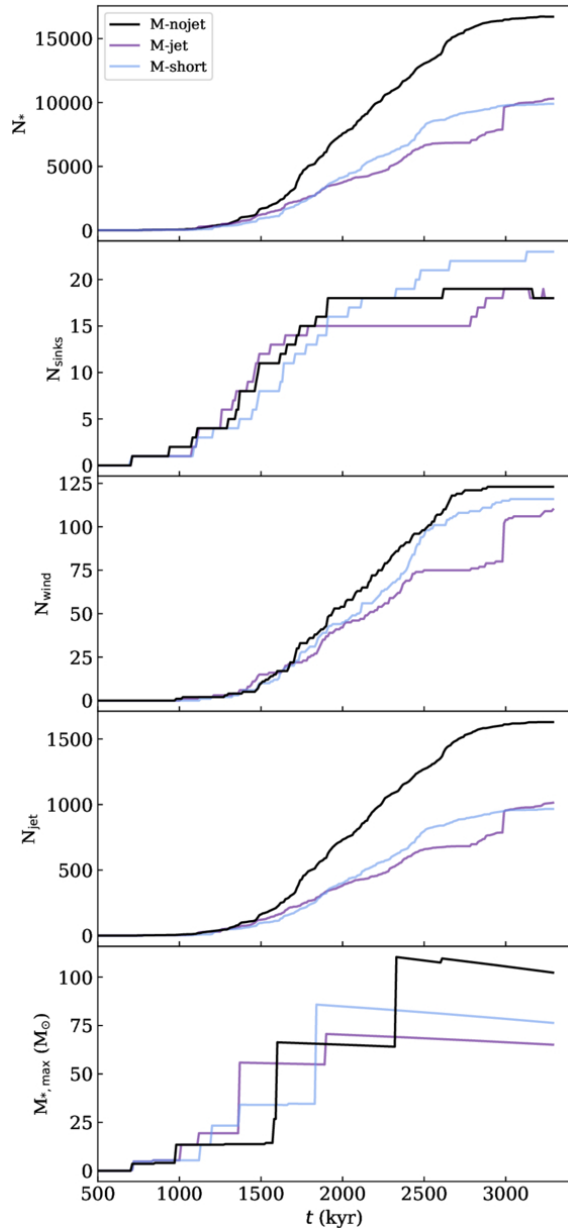
Figure 8. from Sabrina M. Appel et al 2026 Astron. J. 172 doi:10.3847/1538-3881/ae633f https://dx.doi.org/10.3847/1538-3881/ae633f © 2026. The Author(s). Published by the American Astronomical Society.
