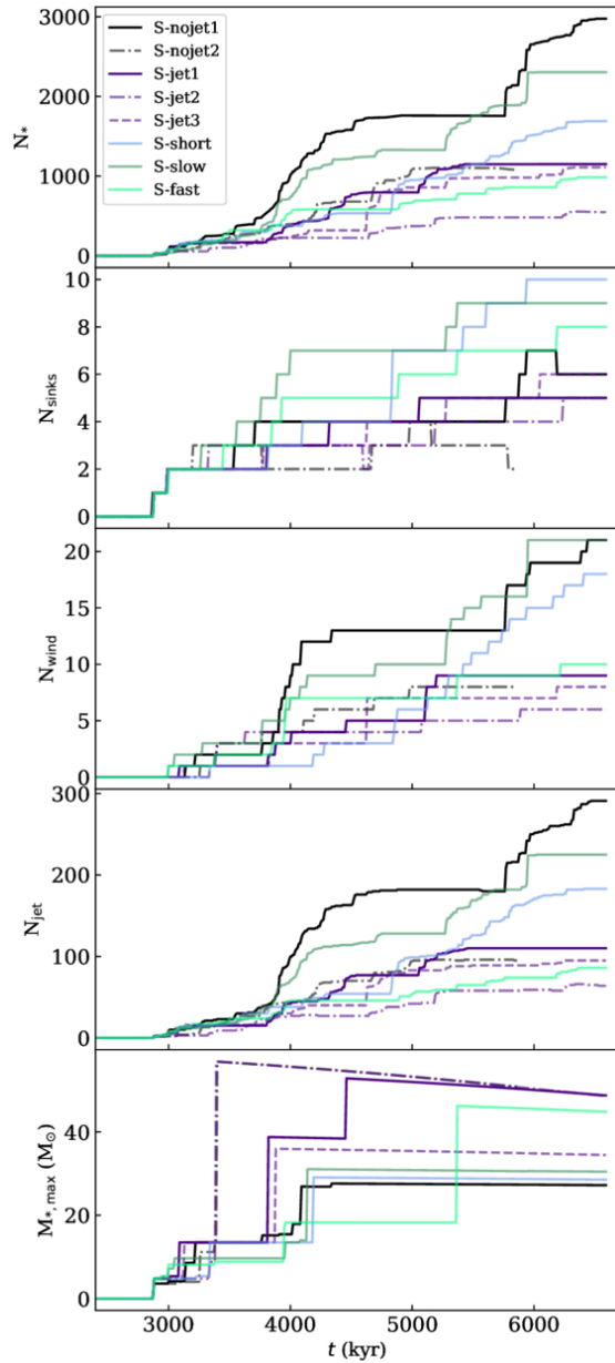
Figure 5. from Sabrina M. Appel et al 2026 Astron. J. 172 doi:10.3847/1538-3881/ae633f https://dx.doi.org/10.3847/1538-3881/ae633f © 2026. The Author(s). Published by the American Astronomical Society.
