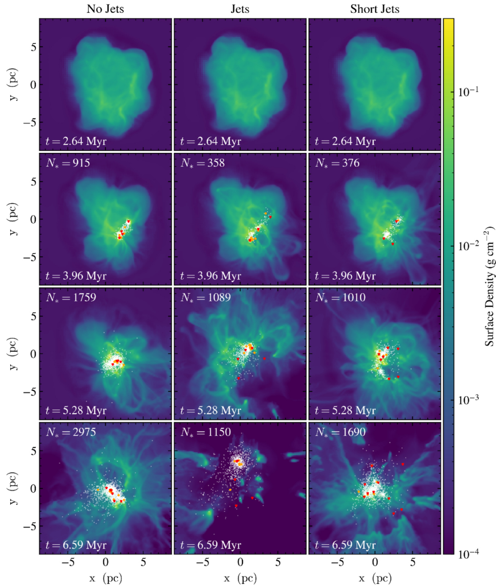
Figure 3. from Sabrina M. Appel et al 2026 Astron. J. 172 doi:10.3847/1538-3881/ae633f https://dx.doi.org/10.3847/1538-3881/ae633f © 2026. The Author(s). Published by the American Astronomical Society.
