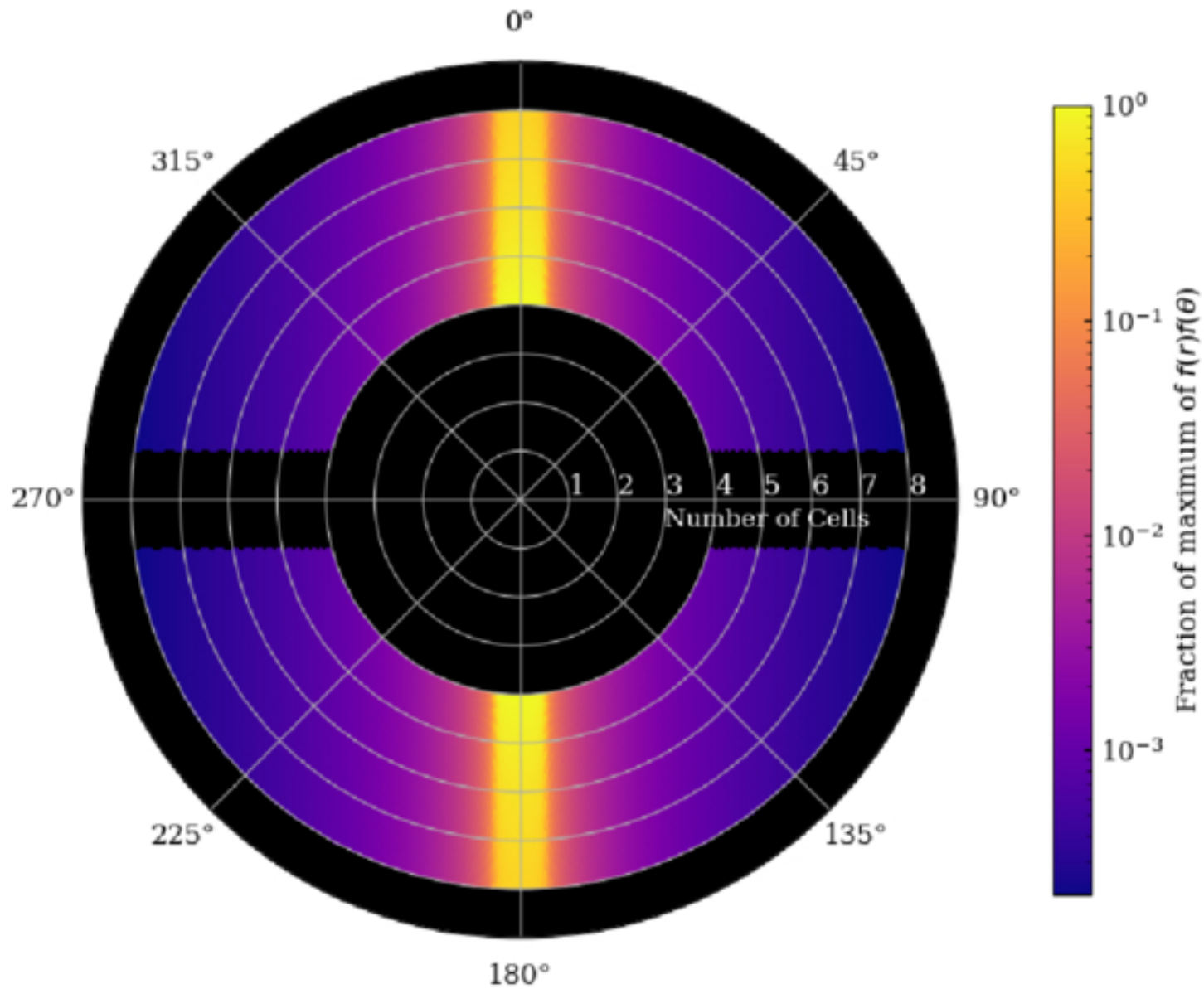
Figure 2. from Sabrina M. Appel et al 2026 Astron. J. 172 doi:10.3847/1538-3881/ae633f https://dx.doi.org/10.3847/1538-3881/ae633f © 2026. The Author(s). Published by the American Astronomical Society.
