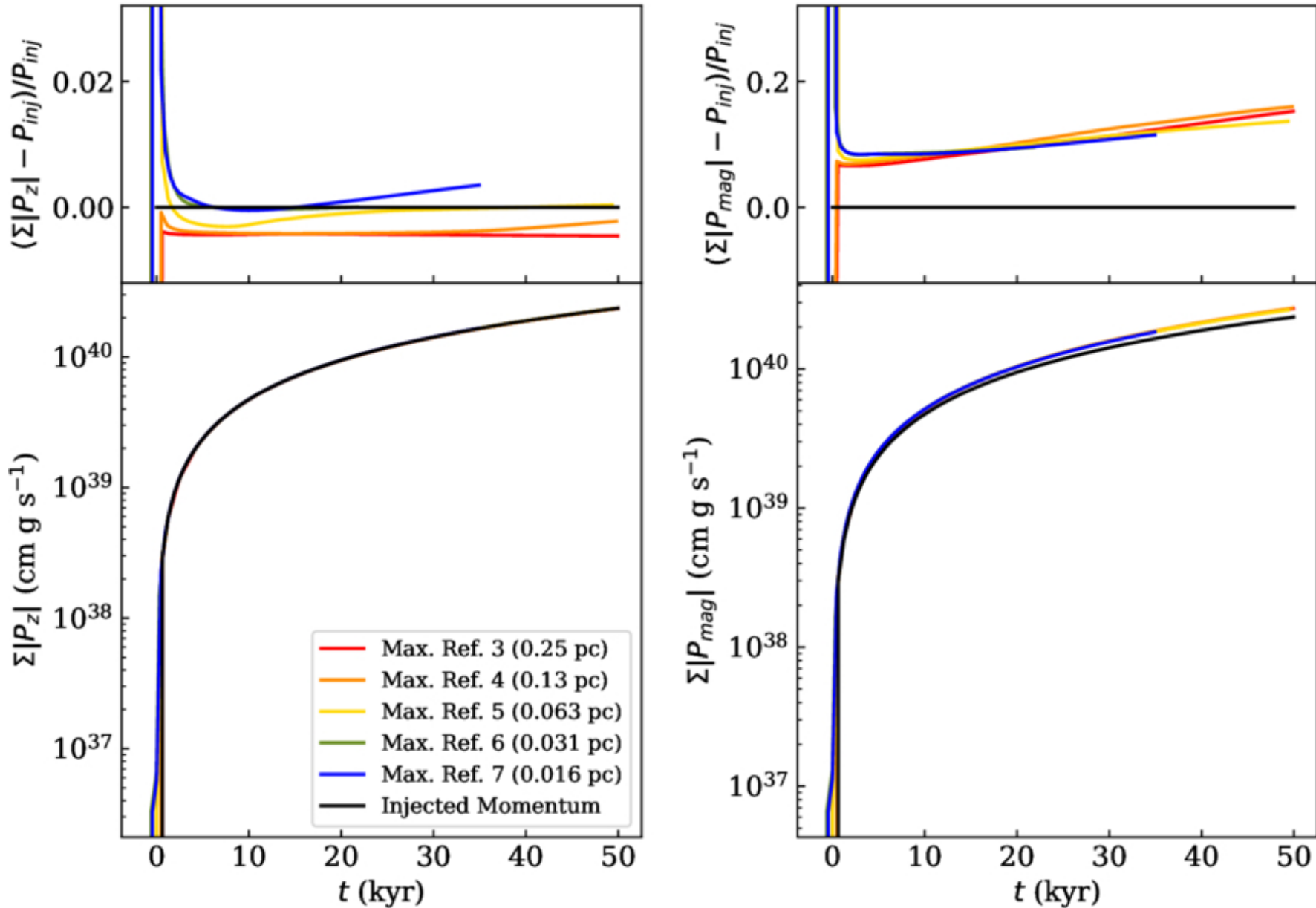
Figure 11. from Sabrina M. Appel et al 2026 Astron. J. 172 doi:10.3847/1538-3881/ae633f https://dx.doi.org/10.3847/1538-3881/ae633f © 2026. The Author(s). Published by the American Astronomical Society.
