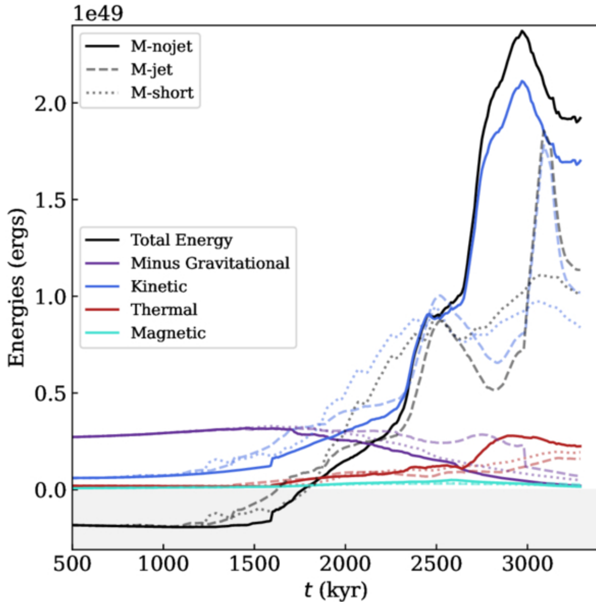
Figure 10. from Sabrina M. Appel et al 2026 Astron. J. 172 doi:10.3847/1538-3881/ae633f https://dx.doi.org/10.3847/1538-3881/ae633f © 2026. The Author(s). Published by the American Astronomical Society.
