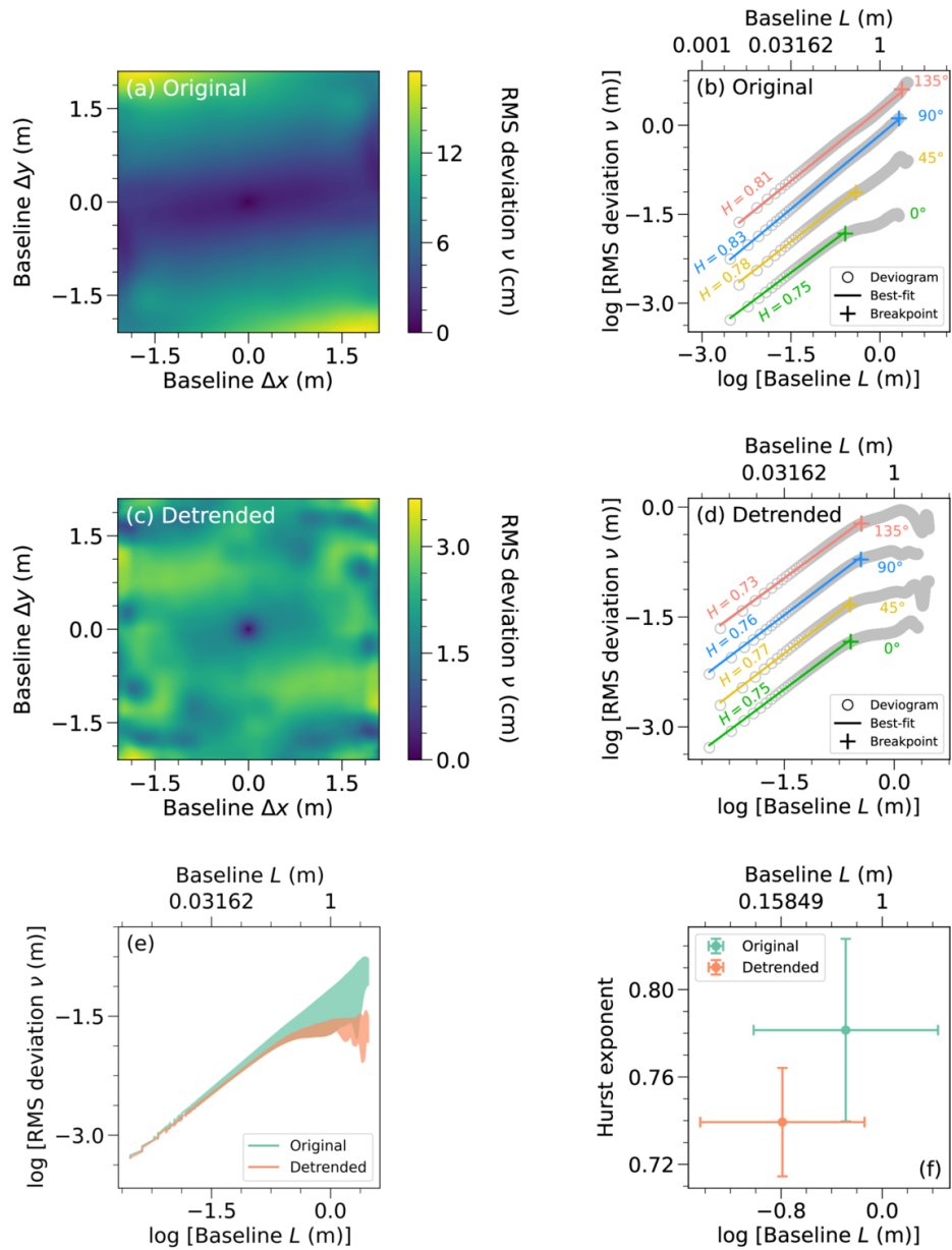
Figure A14. from Jun Du et al 2026 Astron. J. 171 doi:10.3847/1538-3881/ae6333 https://dx.doi.org/10.3847/1538-3881/ae6333 © 2026. The Author(s). Published by the American Astronomical Society.
