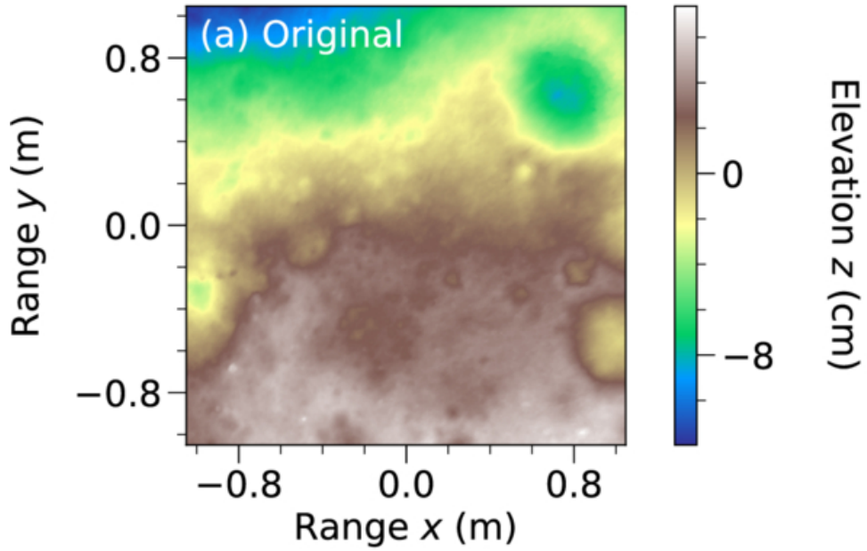
Figure A13. from Jun Du et al 2026 Astron. J. 171 doi:10.3847/1538-3881/ae6333 https://dx.doi.org/10.3847/1538-3881/ae6333 © 2026. The Author(s). Published by the American Astronomical Society.
