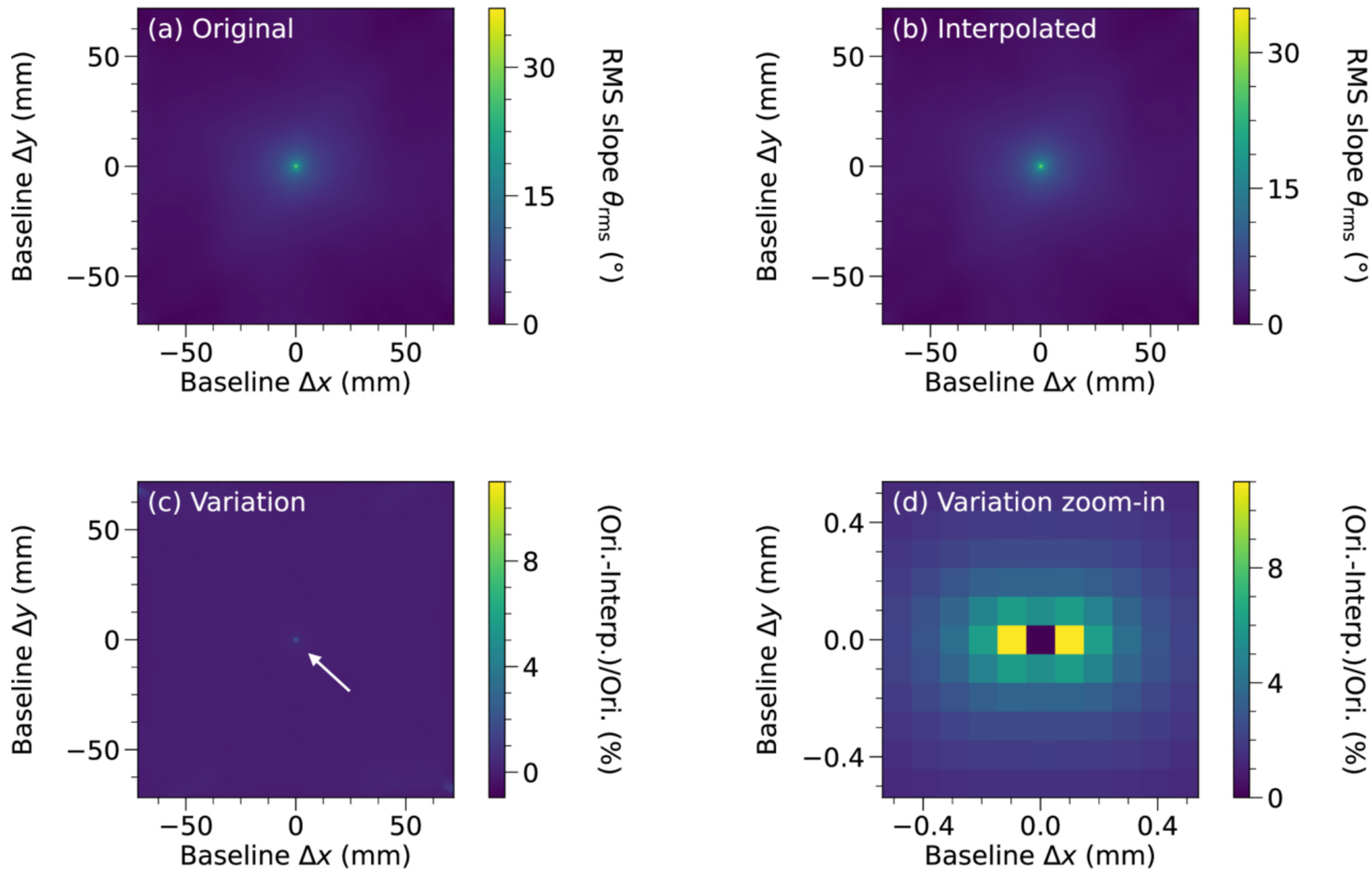
Figure A12. from Jun Du et al 2026 Astron. J. 171 doi:10.3847/1538-3881/ae6333 https://dx.doi.org/10.3847/1538-3881/ae6333 © 2026. The Author(s). Published by the American Astronomical Society.
