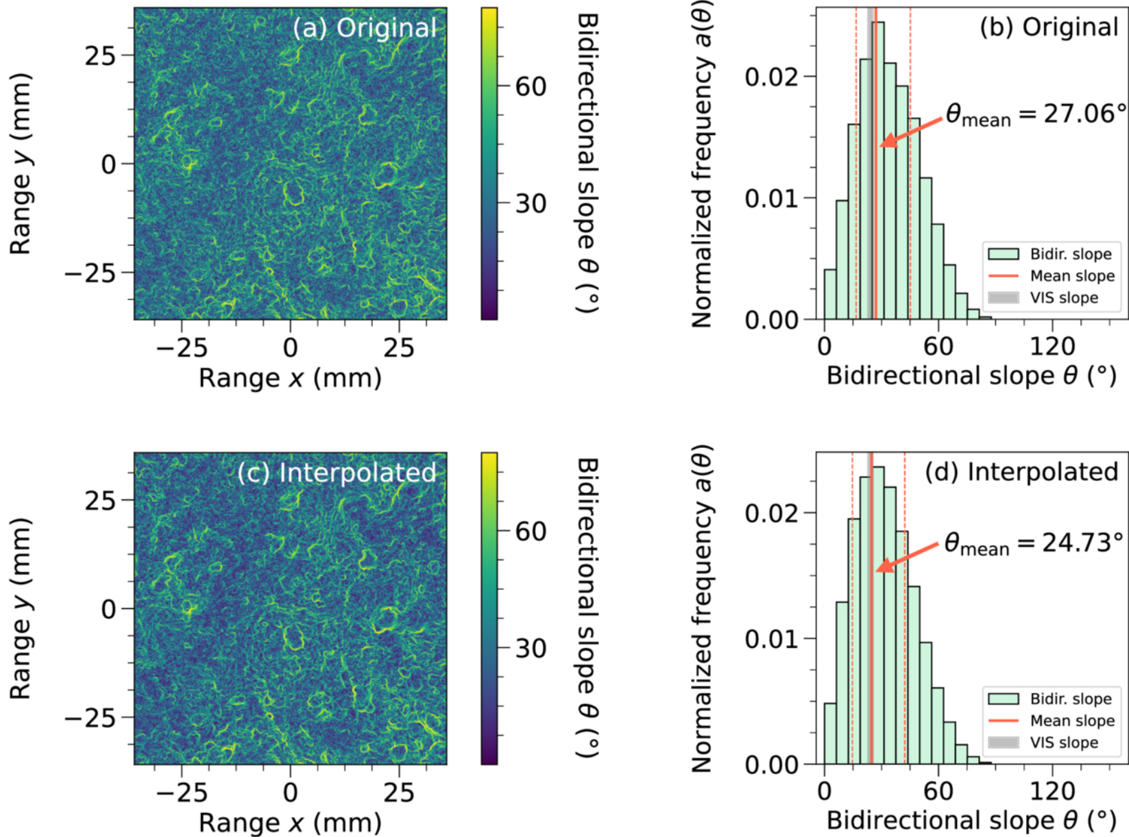
Figure A11. from Jun Du et al 2026 Astron. J. 171 doi:10.3847/1538-3881/ae6333 https://dx.doi.org/10.3847/1538-3881/ae6333 © 2026. The Author(s). Published by the American Astronomical Society.
