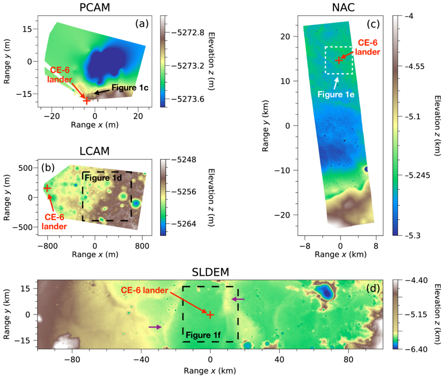
Figure 2. from Jun Du et al 2026 Astron. J. 171 doi:10.3847/1538-3881/ae6333 https://dx.doi.org/10.3847/1538-3881/ae6333 © 2026. The Author(s). Published by the American Astronomical Society.
